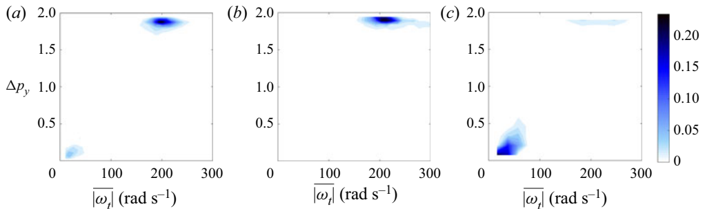
Figure 18. The JPDP of \Delta p_y values versus trajectory-averaged angular velocity for long trajectories of (a) 1 mm, (b) 2 mm and (c) 3 mm disks.
