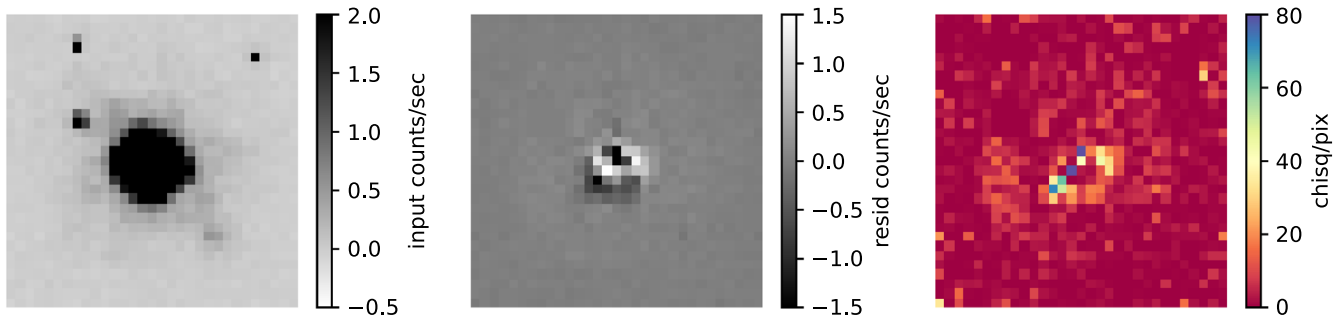
Figure 4. The model-fitting process for the HST exposures is shown for a random exposure, idl004icq . At left is the processed image from MAST, with CTE correction applied. At center are the residuals to a model of a PSF for Dysnomia (to the lower right of Eris in this image) and a disk-broadened PSF for Eris. At right, the residuals are re-plotted as the \chi^2 per pixel using the pixel uncertainties reported by MAST. The residuals in the core of Eris are substantially larger than the statistical errors in the signal, due to the limitations of the PSF models. The residual fluxes can be compared to Eris’s total flux of \approx 800 counts \text{s}^{-1} .
