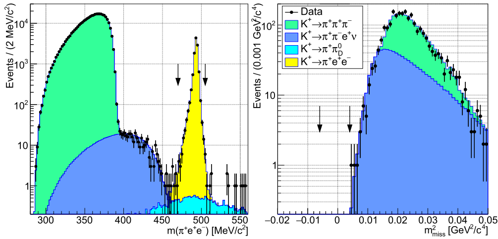
Fig. 2. Left: reconstructed m_{\pi ee} spectra for the data and MC samples obtained with the K_{\pi ee} selection. The data events are not weighted (see Section 3). Right: reconstructed m^2_{\text{miss}} spectra for the data and MC samples obtained with the K_{\mu vee} selection. The normalisation and signal mass regions are indicated by vertical arrows.
