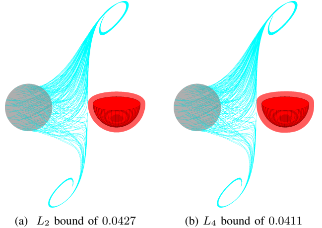
Fig. 4: Twist system trajectories and degree-5 distance bound sublevel sets (20)
