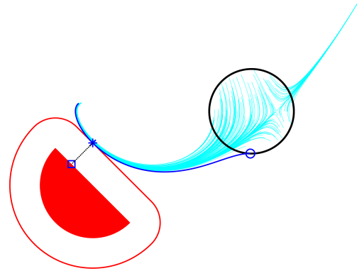
Fig. 2: Flow system trajectories remain at least an L_2 bound of 0.2831 away from X_u
