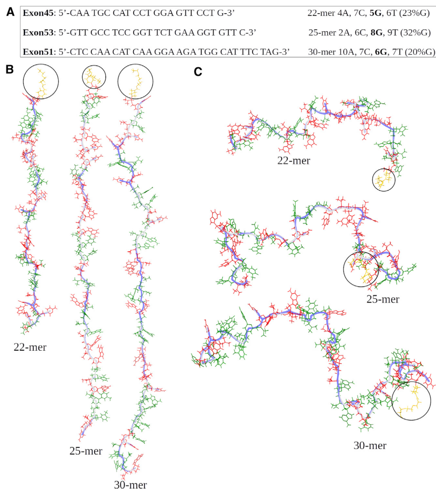
Figure 1. 22-mer, 25-mer, and 30-mer PMO structures
