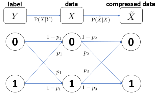
Fig. 2. Transition probabilities for binary data.
