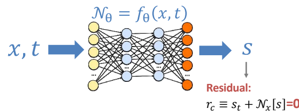
Figure 2. Schematic of PDE solution approximation.
