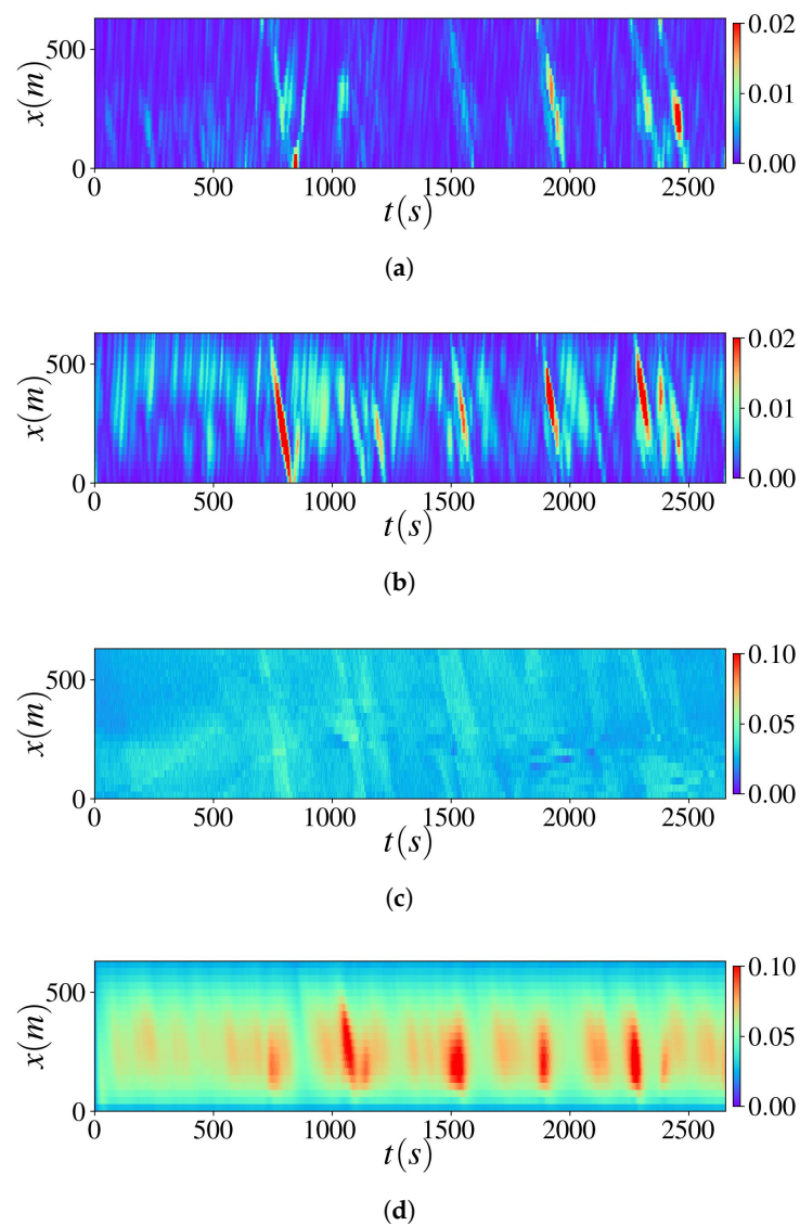
Figure A2. Error heatmaps of the EKF and TrafficFlowGAN. (a) SE_\rho(x, t) of the TrafficFlowGAN; (b) SE_\rho(x, t) of the EKF; (c) prediction's standard deviation of the traffic density of the TrafficFlowGAN; (d) prediction's standard deviation of the traffic density of the EKF.
