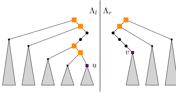
Fig. 6. The invariant: the current search nodes are u and v . uStack contains all nodes on the path from the root to u where the path goes to a right child (orange squares), vStack contains all nodes from the root to v where the path goes to a left child (orange squares). The final leaves u^* and v^* are in one of the gray subtrees; and at least one of them is under u or under v .
