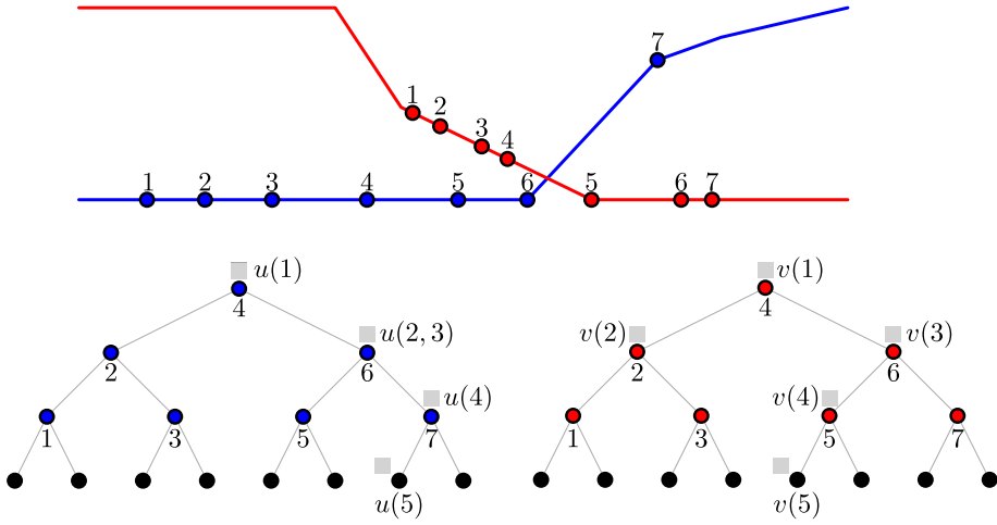
Fig. A.2. Top: the two lower envelopes \mathcal{L}_l and \mathcal{L}_r for the pseudo-lines in Figure A.1. Bottom: the corresponding trees \Delta_l and \Delta_r . The labels u(i) and v(i) indicate the position of the pointers u and v at step i , during the search.
