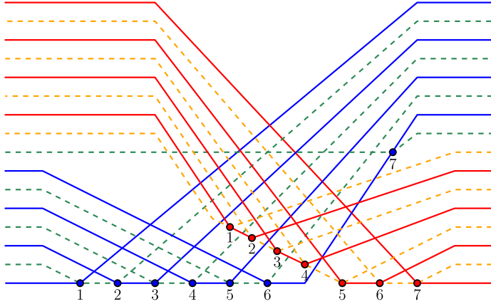
Fig. A.1. Two sets of pseudo-lines and their lower envelopes: (i) the blue and green pseudo-lines, (ii) the red and orange pseudo-lines. The blue and the red dots represent the vertices on the lower envelopes.
