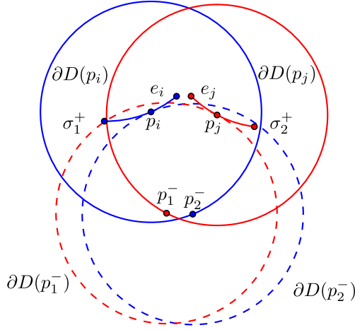
Fig. 14. Illustration of the proof that \gamma_i^- and \gamma_j^- intersect exactly once (see Lemma 3.8).
