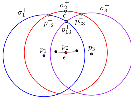
Fig. 15. Illustration of the proof of Lemma 3.9.
