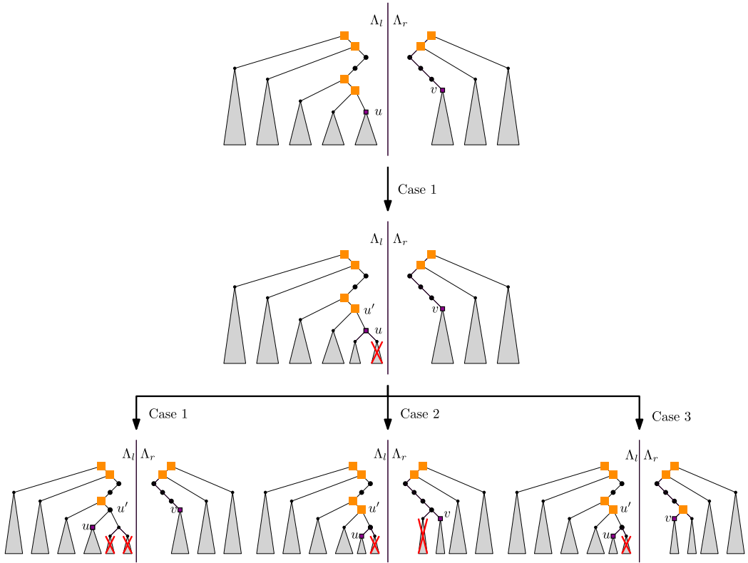
Fig. 7. Comparing u to v : in Case 1, we know that u^* cannot be in u.r . We compare u' and v to decide how to proceed: in Case 1, we know that u^* cannot be in u'.r ; we go to u'.l ; in Case 2, we know that u^* cannot be in u.r and that v^* cannot be in v.l ; we go to u.l and to v.r ; in Case 3, we know that u^* is in u'.r (and hence in u.l ) or in v.l ; we go to u.l and to v.l . Case 2 is not shown, as it is symmetric.
