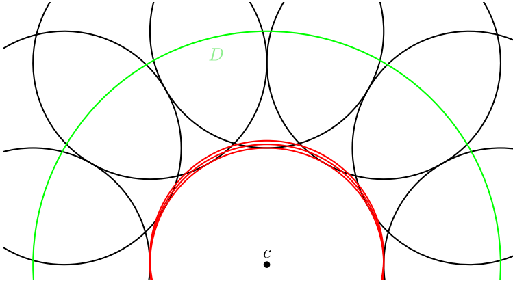
Fig. 1. An instance in which the union boundary of a set of unit discs in the plane undergoes \Omega(n^2) combinatorial changes during n insertions. The black discs are inserted first, and then red discs are inserted from bottom to top.
