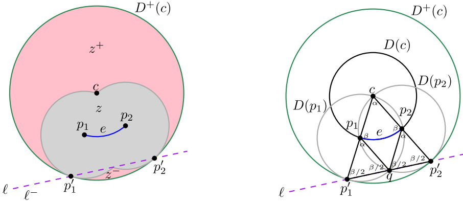
Fig. 17. (On the left) Partition of D^+(c) into three regions: z^+ , z and z^- . (On the right) Illustration of Lemma 4.1.
