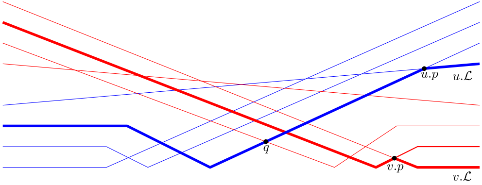
Fig. 3. An example of Case 1: The pseudo-lines in \Lambda_l are shown in blue, the pseudo-lines in \Lambda_r are shown in red.
