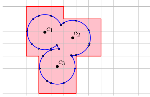
Fig. 8. The grid imposed over the union of unit discs. The active cells are highlighted in pale red.
