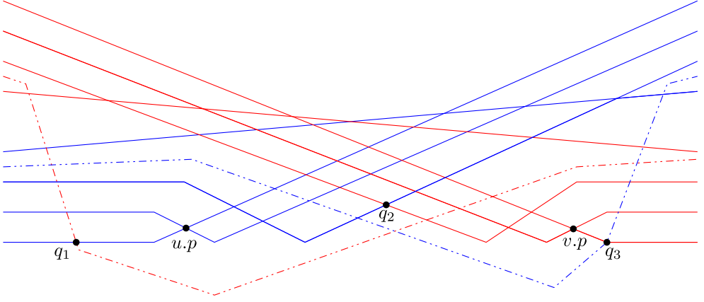
Fig. 4. An example of Case 3: The pseudo-lines in \Lambda_l (resp. \Lambda_r ) are shown in blue (resp. red). The solid pseudo-lines are fixed. The dashed pseudo-lines are optional, meaning that either none or exactly one of the dashed pseudo-lines is present. The current vertices of the binary search are u.p and v.p , and Case 3 applies. Irrespective of the local situation at u and v , the intersection point q of \mathcal{L}_l and \mathcal{L}_r might be to the left of u.p (e.g., q_1 in the figure), between u.p and v.p (e.g., q_2 in the figure), or to the right of v.p (e.g., q_3 in the figure), depending on which one of the dashed pseudo-lines is present.
