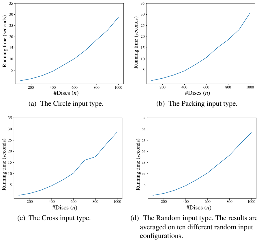
Fig. 15 Running time of the heuristic as a function of the number of discs in the start (and hence also the target) configuration, for the different input types. Each entry ( \# \text{ Discs} = 100, 200, \dots, 1,000 ) in the first three graphs is the average running time of ten different runs, in each of which a different direction \delta is sampled uniformly at random. In the fourth graph (Random input), each entry is the average on ten random inputs, each run ten times on different directions
