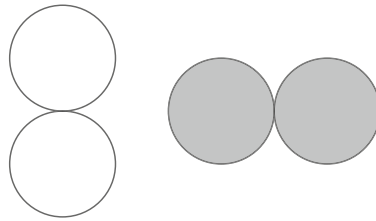
Fig. 1 An infeasible instance for the stationary unlabeled (or labeled) version. The discs of D(S) are drawn empty while the discs of D(T) are drawn shaded
