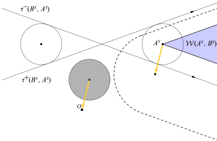
Fig. 4 The vippodrome \mathcal{V}_{AB}^{(1)} , which is the region to the right of the dashed curve in the translation plane. The wedge \mathcal{W}(A^S, B^S) is colored in blue. The vippodrome is obtained by first expanding \mathcal{W}(A^S, B^S) by D_2(o) , and then by shifting by the vector -B^T (in orange)
