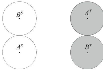
Fig. 3 An infeasible instance for the labeled version: no valid itinerary exists between S and T + \vec{v} , for any translation \vec{v}
