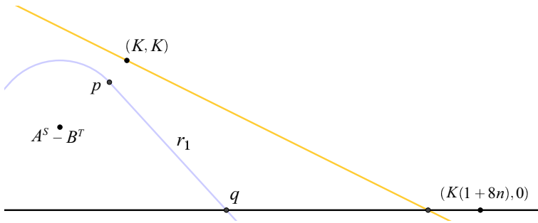
Fig. 14 The x -axis is drawn in black, a bad vippodrome \mathcal{V}_{AB}^{(1)} in blue. The orange line, with slope -\tan(\pi/(24n)) , meets the x -axis to the right of any bad vippodrome of the first type, which is directed downwards (and to the left), like \mathcal{V}_{AB}^{(1)}
