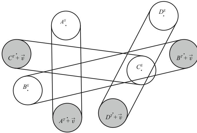
Fig. 2 The hippodromes H_{\vec{v}} for four pairs A, B, C, D \in M and some fixed \vec{v} . Notice that even though H_{\vec{v}}(A) \cap H_{\vec{v}}(B) \neq \emptyset , there is no restriction that the motion of A must precede or succeed the motion of B . Such restrictions do exist for many other pairs, such as B and C ( C has to perform a motion before B )
