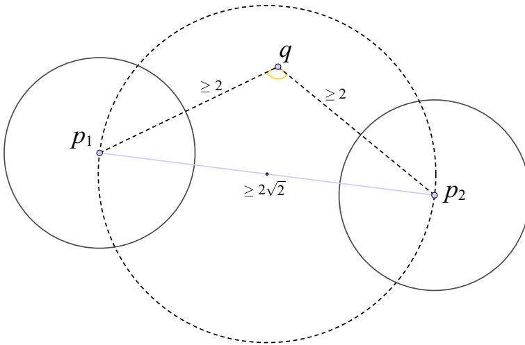
Fig. 13 The segment p_1p_2 (in blue) is not a Delaunay edge, so its diametral disc contains another point q \in S , and then \angle p_1qp_2 \geq \pi/2
