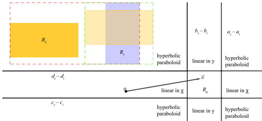
Fig. 9 An example of \text{AABR}(D(S)) (in blue), \text{AABR}(D(T)) (in orange) and \text{AABR}(D(T + \vec{v})) (in light orange) for some \vec{v} \in R_0 . The lines of L partition the translation plane into nine regions, in each of which \varphi behaves differently, as indicated. The boundaries of \text{AABR}(D(S) \cup D(T)) and \text{AABR}(D(S) \cup D(T + \vec{v})) are depicted by red and green dashed contours, respectively. Observe that \text{AABR}(D(S) \cup D(T + \vec{v})) is of minimal area
