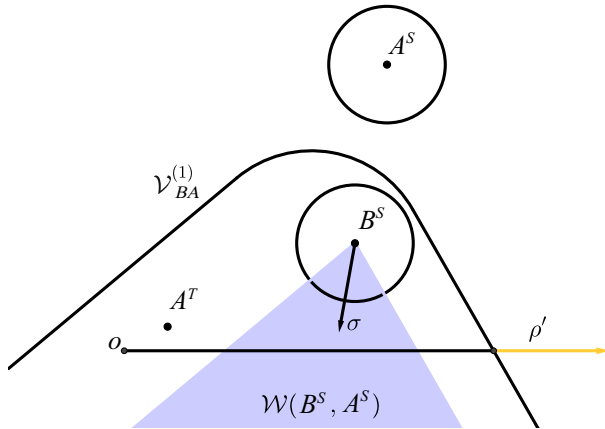
Fig. 12 According to \Pi(M_\delta) , A preforms a motion before B . Therefore, we need to rule out translations \vec{v} for which B has to perform a motion before A , whose locus is exactly the bad vippodrome \mathcal{V}_{BA}^{(1)} . Here \delta is horizontal and points to the right. The wedge \mathcal{W}(B^S, A^S) (in blue), and thus also the bad vippodrome, cannot fully contain \rho , and thus there exists \rho' (in orange) that is disjoint from the vippodrome
