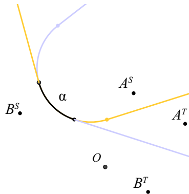
Fig. 5 The vippodromes \mathcal{V}_{AB}^{(1)} and \mathcal{V}_{AB}^{(2)} , colored in blue and orange, respectively. The arc \alpha is the overlap portion of the two vippodrome boundaries
