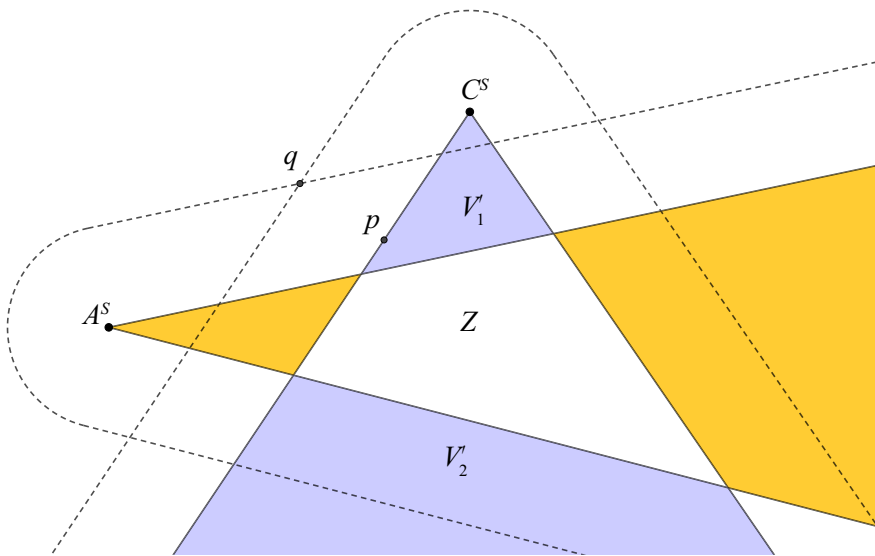
Fig. 8 Two vippodrome boundaries \partial\mathcal{V}_{AB}^{(1)} and \partial\mathcal{V}_{CD}^{(1)} marked by dashed curves. V' and U' = U \setminus Z are colored in blue and orange, respectively. Note that p cannot lie on \partial Z
