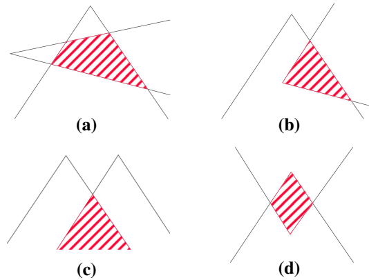
Fig. 7 Some of the possible intersections of U and V , with the intersection Z highlighted. In all cases, V' consists either of one non-convex connected component, see (b) and (d), or of at most two convex connected components, see (a) and (c)
