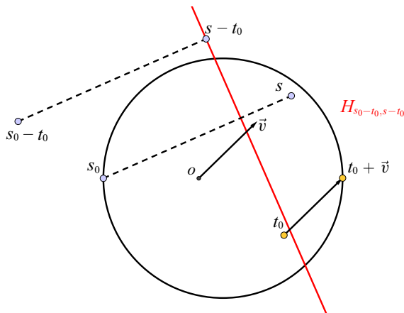
Fig. 11 The points s_0, s (in blue), t_0 (in orange), and their respective translated points according to -t_0 and \vec{v} . The halfplane H_{s_0-t_0, s-t_0} , lies to the right of its bounding line, which is marked in red. Observe that \vec{v} \in H_{s_0-t_0, s-t_0} and so s is inside the diametral disc of s_0 and t_0 + \vec{v}
