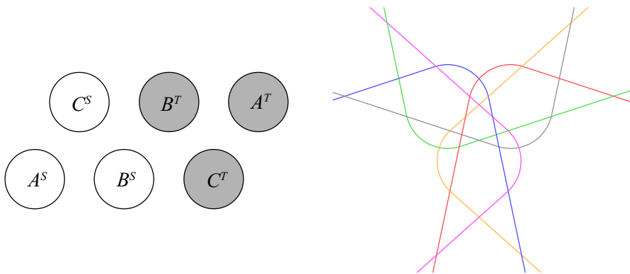
Fig. 6 A scenario where no valid translation exists. Left: The start and target configurations. Right: All the 12 vippodromes are drawn (in the translation plane). Observe that the vippodromes \mathcal{V}_{AB}^{(2)} and \mathcal{V}_{BA}^{(1)} coincide (their boundaries are drawn in orange), and so does every other similar pair of vippodromes for the other pairs of positions. Each point in the translation plane is covered by at least two vippodromes of contradicting constraints (e.g., for points inside the orange vippodrome, A has to perform a motion before B and vice versa), and so every translation is invalid (its TBG contains a 2-cycle)
