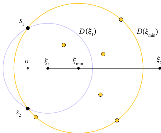
Fig. 10 The origin o is the midpoint of s_1s_2 . The points of T + \vec{v} are drawn in orange. The other points of S are not drawn, but they lie in all the discs D(\xi) , for \xi \in [\xi_1, \xi_2] . D(\xi_1) (in blue) is the smallest enclosing disc of S among those centered on the Voronoi edge e_{s_1, s_2} = [\xi_1, \xi_2] . D(\xi_{\min}) (in orange) is the smallest enclosing disc of S \cup (T + \vec{v}) whose center lies on e_{s_1, s_2}
