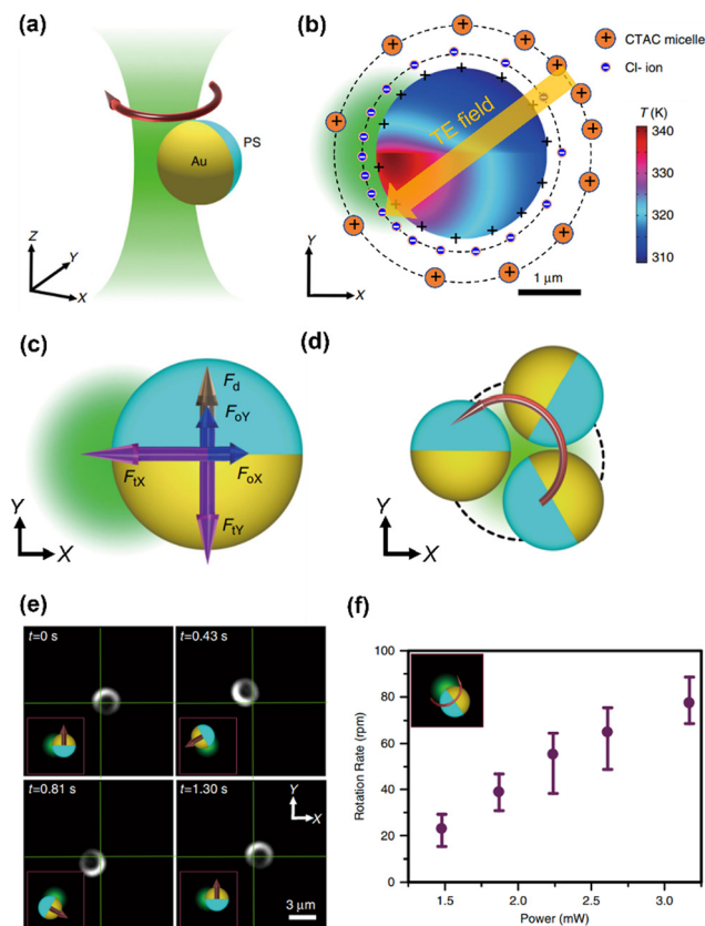
Fig. 4 The opto-thermoelectric rotation technique. (a) 3D schematic illustration of an orbiting metal-coated Janus particle driven by a laser beam. (b) Simulated temperature distribution of a 2.7 μm Au/PS Janus particle under the illumination of a 532 nm beam at a power of 2 mW. The distribution of ions and the established thermoelectric field are illustrated as well. The orange and blue solid circles represent the CTAC micelles and Cl - ions, respectively. The orange arrow denotes the direction of the thermoelectric field. (c) Schematics of the thermoelectric force (purple), optical force (blue), and drag force (brown) acting on the Janus particle. (d) Two-dimensional (2D) schematics of the orbital movements of the particle powered by the beam. (e) Time-resolved dark-field images of the rotation of the Janus particle. (f) The measured rotation rate as a function of the optical power of the beam. Adapted with permission. 98 Copyright 2020, Springer Nature.
