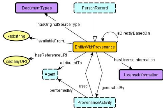
Fig. 3. Schema diagram for the Provenance module from the Enslaved Ontology [44]. It is based on the Provenance pattern from [20], which in turn is based on the core of PROV-O [45].
