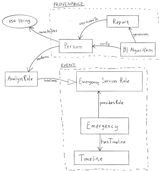
Fig. 11. Task A Schema Diagram
