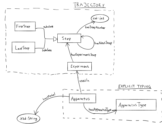
Fig. 12. Task B Schema Diagram
