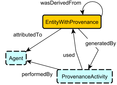
Fig. 4. Schema diagram of the MODL Provenance ODP. It is based on the core of PROV-O [45]
