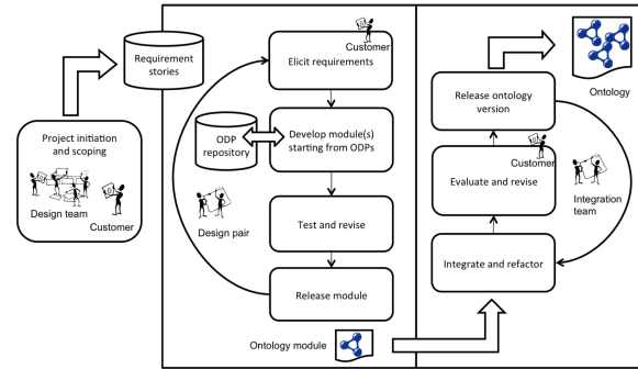
Fig. 1. eXtreme Design method overview, from [17].
