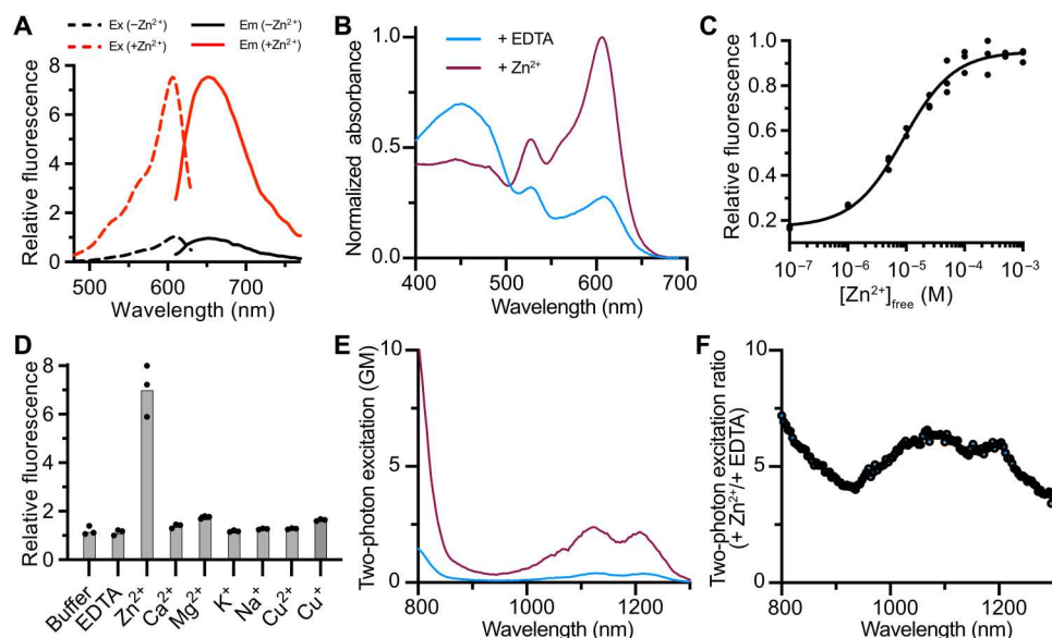
Fig. 2. Spectroscopic characterization of FRISZ as a purified protein. (A) Excitation (dashed line) and emission (solid line) spectra of purified FRISZ in the presence of 100 \mu\text{M} \text{Zn}^{2+} (red) or 100 \mu\text{M} EDTA (black). (B) One-photon absorbance spectra of FRISZ in the presence of 100 \mu\text{M} \text{Zn}^{2+} or 100 \mu\text{M} EDTA. (C) Dose-response curve of purified FRISZ ( K_d = 8.8 \pm 1.0 \mu\text{M} , n = 3 ). (D) Fluorescence of FRISZ in response to \text{Zn}^{2+} and other indicated chemicals (100 \mu\text{M} , n = 3 ). (E) Two-photon fluorescence excitation spectra of FRISZ in the presence of 100 \mu\text{M} \text{Zn}^{2+} or 100 \mu\text{M} EDTA. (F) The ratio of two-photon excitation plotted against wavelength.
