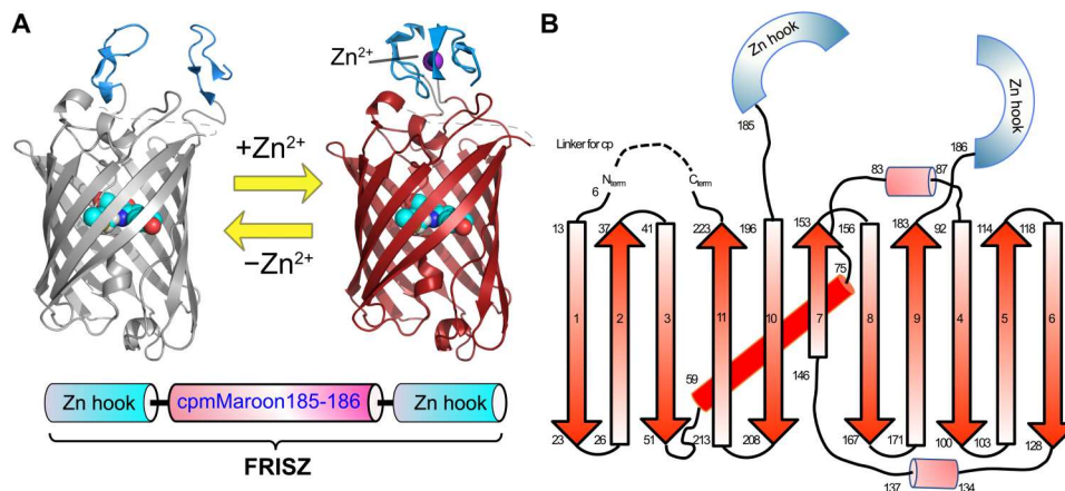
Fig. 1. Illustration of the \text{Zn}^{2+} -sensing mechanism and the secondary structure of FRISZ. (A) Illustration of FRISZ, in which two Rad50 zinc hook motifs are fused to the N and C termini of cpMaroon185-186. The domain arrangement of the primary sequence is also presented at the bottom. (B) Schematic representation of the secondary structure elements of FRISZ. Secondary structure elements in cpmMaroon185-186 are based on a mMaroon1 structure predicted by SWISS-MODEL using mCardinal (Protein Data Bank: 4OQW) as the template. Cylinders represent \alpha helices, and arrows represent \beta strands. The Rad50-derived zinc hook motifs are presented as blue semicircles.
