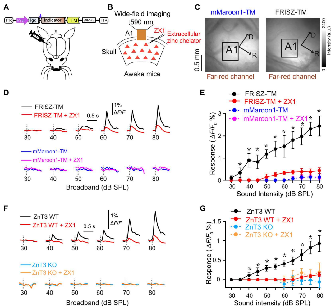
Fig. 5. Imaging of synaptic \text{Zn}^{2+} with FRISZ-TM, in response to sound stimuli in awake mice. (A) Schematics of AAV genetic elements and injection into mouse AC. (B) Illustration of transcranial imaging of FRISZ-TM or mMaroon1-TM in head-fixed awake mice. ZX1 was infused into the AC via a glass pipette connected to a syringe pump. (C) Fluorescence images of the primary AC (A1) showing the expression of mMaroon1-TM (left) and FRISZ-TM (right). D, dorsal; R, rostral. (D) Representative transcranial FRISZ-TM (top) or mMaroon1-TM (bottom) fluorescence signals in response to broadband sounds before (black or blue) and after (red or magenta) ZX1 infusion in C57BL/6J mice. (E) Summary plot of average sound-evoked fluorescence signals of FRISZ-TM (n = 5) and mMaroon1-TM (n = 3) in C57BL/6J mice. (FRISZ-TM: control versus ZX1; two-way ANOVA; effect of ZX1, F = 12.01 , P = 1.0 \times 10^{-6} ; *P < 0.05 , compared to ZX1, Holm-Bonferroni's post hoc). Dotted lines represent nonsignificant responses. (F) Representative transcranial FRISZ-TM fluorescence signals to broadband sounds before (black or cyan) and after (red or orange) ZX1 infusion in ZnT3 WT (top) or KO (bottom) mice. (G) Summary plot of average sound-evoked fluorescence signals from ZnT3 WT (n = 4) and KO (n = 4) mice. (ZnT3 WT: control versus ZX1; two-way ANOVA; effect of ZX1, F = 16.02 , P = 0.02 ; *P < 0.05 , compared to ZX1, Holm-Bonferroni's post hoc). Dotted lines represent nonsignificant responses. See table S1 for statistical details. Error bars indicate SEM.
