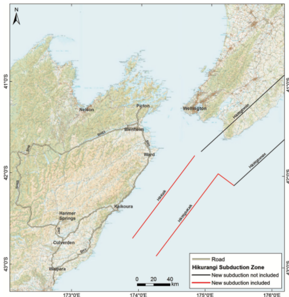
Figure 11. The extensions of the Hikurangi subduction interface sources from those of the 2010 NSHM (Stirling et al. 2012). The traces of the top edges of the new KSHM segments are shown in red, and those of 2010 NSHM sources in black. All sources dip at shallow angles to extend at depth under the land.
