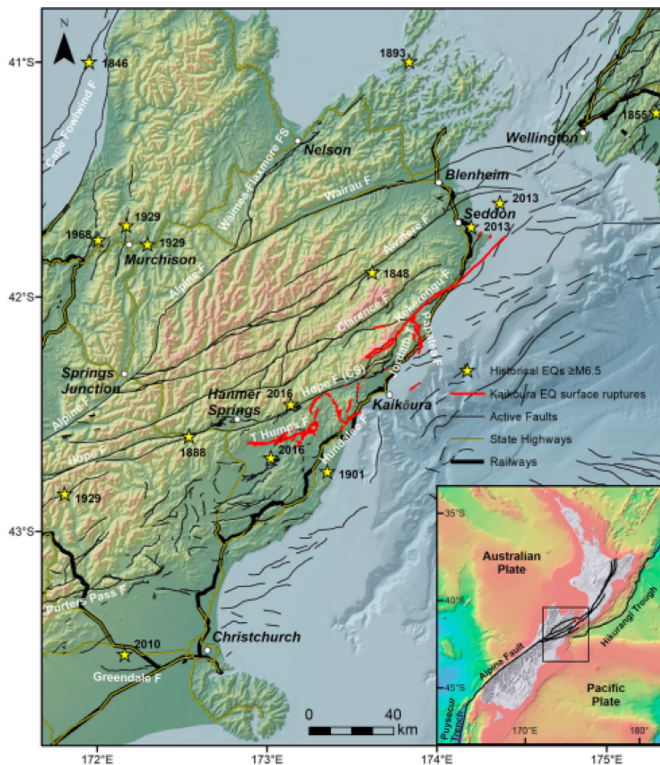
Figure 1. A, Active faults, epicentres of historical (post-1840 AD) earthquakes with M_w \geq 6.5 and the main road and railway networks in central New Zealand. Onshore active faults (including the Kaikōura Earthquake ground surface ruptures) are from the New Zealand Active Faults Database ( https://data.gns.cri.nz/af/ ; Langridge et al. 2016). Selected major faults are named. Offshore active faults are from Barnes et al. (2010, 2016), Mountjoy et al. (2009), Pondard and Barnes (2010). Earthquake epicentres, labelled with the earthquake year, are from the GeoNet earthquake catalogue ( https://www.geonet.org.nz/data/types/eq_catalogue ). The basemaps are hillshade and digital elevation models from the 8 m 2012 UNZ (onshore; https://data.lin.govt.nz/layer/51768-nz-8m-digital-elevation-model-2012/ ) and the 250 m 2016 NIWA bathymetry (offshore; https://data-niwa.opendata.arcgis.com/datasets/nz-bathymetry-250m-imagery-raster-layer/explore ) datasets. B, Plate boundary setting of central New Zealand. CSHM is the area of the Canterbury Seismic Hazard Model (Gerstenberger et al. 2014, 2016).
