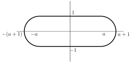
FIG. 4. A stadium-shaped charge distribution. The stadium's aspect ratio is defined as a + 1 , where a denotes the half-length of the straight portion of the stadium.
