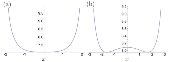
FIG. 6. (a) Potential along x axis for stadium with a = 1 . (b) Potential along x axis for stadium with a = 2 . The three critical points where the slope vanishes correspond to electrostatic equilibrium points, i.e., zeros of the electric field.
