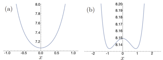
FIG. 3. The potential of charged rectangles along the x axis. (a) Aspect ratio a = 1.1 . The only critical point lies at the origin. (b) Aspect ratio a = 2.5 . The three critical points where the slope vanishes correspond to electrostatic equilibrium points, i.e., zeros of the electric field.
