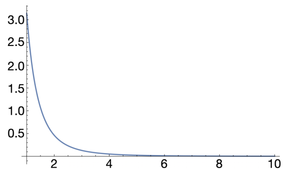
FIG. 7. The second derivative in x of \phi at the origin for a charged ellipse with aspect ratio a . Here a is defined as the length of the ellipse's major axis, measured in units of its minor axis. Numerically, it appears that the second derivative of the potential is strictly positive at the origin. This observation provides numerical evidence that the electric field associated with any charged ellipse has exactly one zero.
