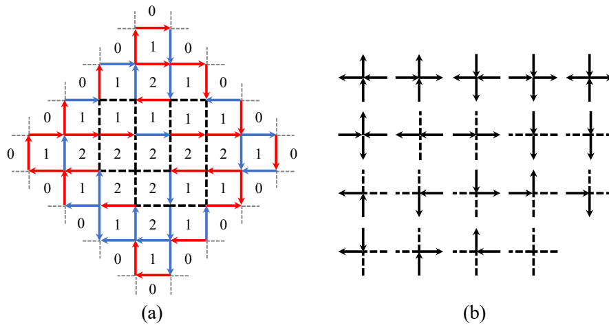
Figure 9: (a) A random coupled Motzkin lattice configuration with Aztec diamond boundary. (b) The 19 vertices in the constrained Hilbert space satisfying equal number of in and out arrows.
