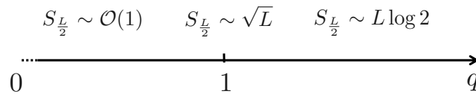
Figure 2: The common entanglement phase diagram of colored Fredkin and Motzkin chains.
