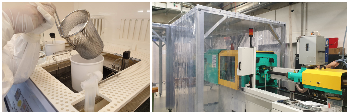
Figure 1. Left: PEN pellets in stainless-steel sieve during cleaning process. The PTFE container is placed in a basin filled with DI water for ultra sound cleaning. Right: injection compression molding machine used for production of PEN discs. All open parts of the machine are located inside a clean room.
