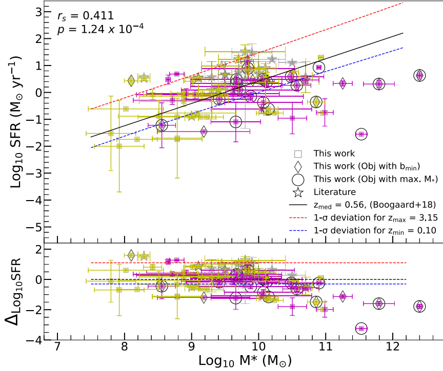
Figure 6. Upper panel: SFR versus stellar mass for galaxies associated with gas-rich absorbers. The grey stars denote galaxies from Zabl et al. (2019) whose H I column density is more uncertain [not based on the actual Ly \alpha absorption profile, but estimated from the Mg II \lambda 2796 equivalent width using the relation from Ménard & Chelouche (2009)]. The yellow and magenta stars denote galaxies from Fynbo et al. (2011), Krogager et al. (2012), Christensen et al. (2014), Augustin et al. (2018), and Rhodin et al. (2021). All other symbols are as in Fig. 5. The solid black line shows the SFMS from Boogaard et al. (2018) at the median redshift of the sample galaxies. The blue and red dashed lines show the 1\sigma deviations from the SFR– M_* relations at z_{\min} and z_{\max} of the full sample of absorber-associated galaxies (including galaxies from both our MAH sample and the literature). Lower panel: plot of the difference between the observed SFR and the expected SFR from the SFMS at z_{\text{med}} taken from Boogaard et al. (2018) at the observed stellar mass versus the stellar mass. The blue and red dashed lines show the difference relative to the SFMS at z_{\text{med}} for the lower and upper 1\sigma SFMS at z_{\min} and z_{\max} .
