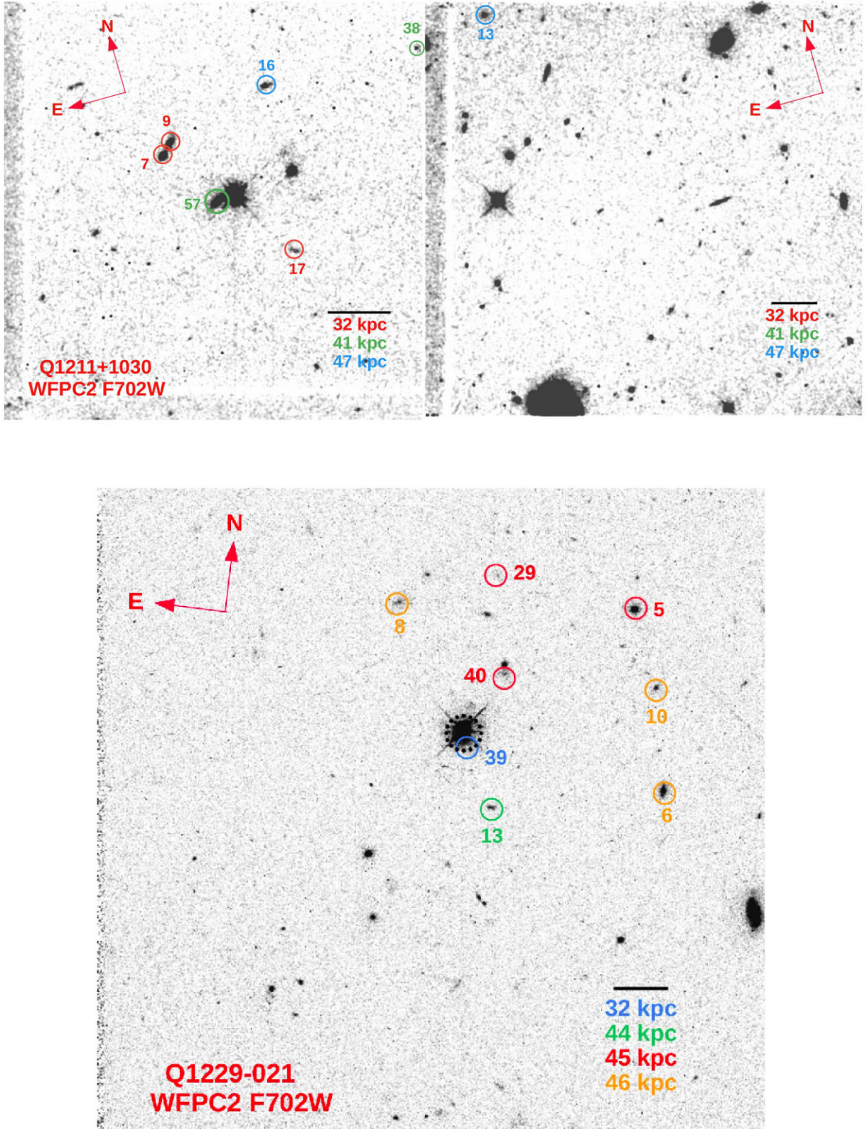
Figure A4. See Fig. A1 caption. The scale bar corresponds to 32, 41, and 47 kpc at z_{\text{abs}} = 0.3929, 0.6296, and 0.8999 for the top figures, while the scale bar corresponds to 32, 44, 45, and 46 kpc at z_{\text{abs}} = 0.3950, 0.7572, 0.7691, and 0.8311 for the bottom figure, respectively.
