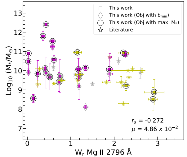
Figure 9. The rest-frame equivalent width of Mg II \lambda 2796 plotted against the stellar mass. All symbols are as in Fig. 5. A tentative negative correlation is seen: more massive galaxies are associated with lower metal line strengths. Such a trend would be consistent with the fact that the stellar mass of the galaxy is anticorrelated with the column density of H I gas (e.g., Augustin et al. 2018), while N_{\text{HI}} is positively correlated with the equivalent width of the Mg II line (e.g., Rao et al. 2006).
