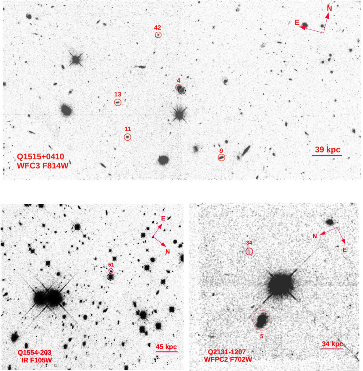
Figure A6. See Fig. A1 caption. The scale bar corresponds to 39 kpc at z_{\text{abs}} = 0.5592 for the top figure, while in the bottom figures, the scale bar corresponds to 45 and 34 kpc at z_{\text{abs}} = 0.7869 and 0.4298 for the left and right figures, respectively.
