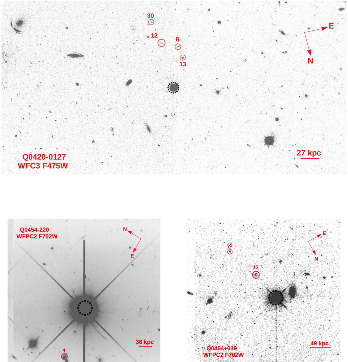
Figure A2. See Fig. A1 caption. The scale bar corresponds to 27 kpc at z_{\text{abs}} = 0.6331 for the top figure, while in the bottom figures, the scale bar corresponds to 36 and 49 kpc at z_{\text{abs}} = 0.4833 and 1.1532 for the left and right figures, respectively.
