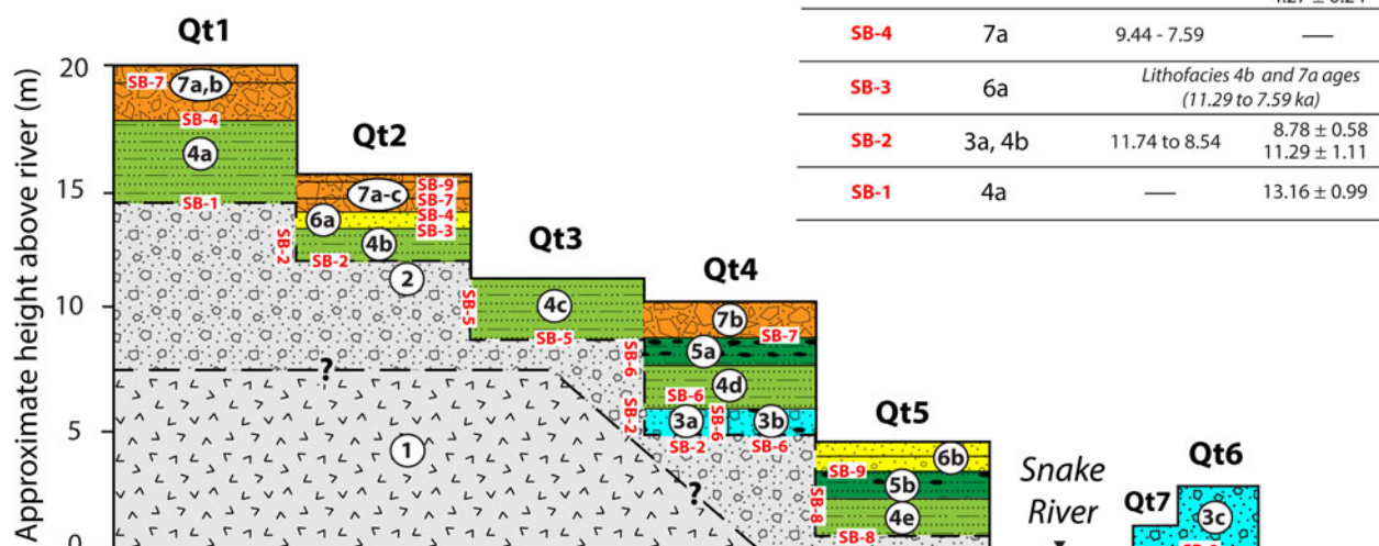
Figure 5. Schematic, composite stratigraphic model of the sequence of cut-and-fill cycles of post-Bonneville fluvial terraces (Qt1–Qt7) and alluvial fan and fluvial/alluvial margin deposition on the middle Snake River at Bancroft Springs. Terrace tread heights, plus stratigraphic and geochronologic relations are developed from natural exposures at 10 study sites (Fig. 3). The radiocarbon and luminescence ages of lithofacies units and sequence boundaries (SB) are also shown.
