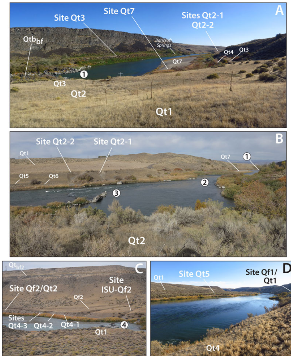
Figure 2. Site photographs within the Bancroft Springs study area (Figs. 1, 3). (A) View upstream to the southeast of the sequence of Qt1–Qt4, Qt6, and Qt7 terrace trends near channel constriction #1 (numbered white circle) composed of boulder-rich Bonneville Flood expansion bar (Qt bf ) in the northern reach of river showing steep canyon walls on east bank composed of intra-canyon lava flows and more subdued walls on west bank composed of the Glens Ferry Formation consisting of interbedded siltstone and sandstone with lava flows. Stratigraphic study sites Qt2-1, Qt2-2, Qt3, and Qt7, along with Bancroft Springs are also shown. (B) View downstream to the north-northwest from east bank on Qt2 terrace showing the prominent terrace tread Qt2 and sites Qt2-1 and Qt2-2 near narrow channel constriction #2 and Bonneville Flood debris that form rapids at channel constriction #3. Terraces Qt1, Qt5–Qt7, and channel constriction #1 are also shown. (C) View across river to the west-southwest showing the canyon wall along west bank of river with inset Qt4 terrace overlain by Qf2 alluvial fan deposit near channel constriction #4 composed of Bonneville Flood debris that forms rapids. Bonneville Flood terrace Qt bf2 , and fluvial Qt1 and Qt2 terraces, along with sites Qf2/Qt2, Qt4-1, Qt4-2, Qt4-3, and ISU-Qf2 are also shown. (D) View upstream to the south-southeast from the west bank on Qt4 terrace showing reaches of Snake River in study area with planar Qt5 terrace tread below Qt1 terrace on east bank of river. Study sites Qf1/Qt1 and Qt5 on bluff exposures are also shown.
