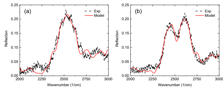
Figure 5. Experimental reflection measurements (black dashed lines) taken before (a) and during (b) compression of the photonic crystal and best-fit models (red solid lines). Measurements were taken through the fused silica window. The feature dominating the spectra was the photonic bandgap, which was centered around 2535\text{ cm}^{-1} . During compression, a transmissive defect resonance was observed within the photonic bandgap. The experimental and best-model calculated reflection data were in good agreement.
