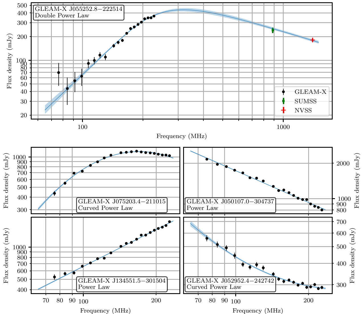
Figure 18. Five example SEDs of sources selected to highlight the variety of spectral shapes seen within the GLEAM-X data. The panel inset includes the source name and model used to fit the presented data. The optimised model and its 1\sigma confidence interval is overlaid as the blue line of each source. The ‘Power Law’ and ‘Curved Power Law’ are defined as Equations (4) and (5), respectively. The ‘Double Power Law’ used for GLEAM-X J055252.8–222514 shows Equation (3) of Callingham et al. (2017) fitted using the GLEAM-X data and higher frequency measurements from SUMSS and NVSS.
