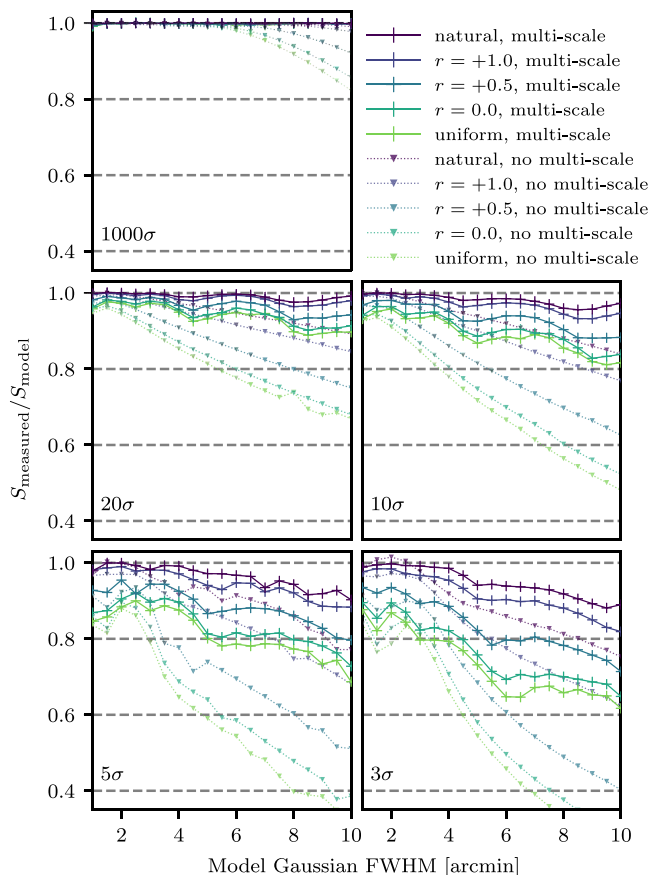
Figure 2. Flux density recovery fraction for model 3, 5, 10, 20, and 1000 \sigma 2-d Gaussian sources with varying FWHM for a range of image weightings. The FWHM range from 60 arcsec up to 600 arcsec in 30 arcsec intervals. The PSF major axis FWHM varies from 80 arcsec (for uniform weighting) to 115 arcsec (for natural weighting). Note the step-pattern visible in the multi-scale cases likely arises due to choice of scales during multi-scale CLEAN.
