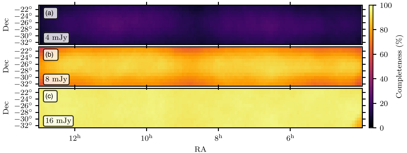
Figure 14. Completeness fraction as a function of position on the sky for three representative cuts in source integrated flux density at 200 MHz, for the catalogue released in this work.
