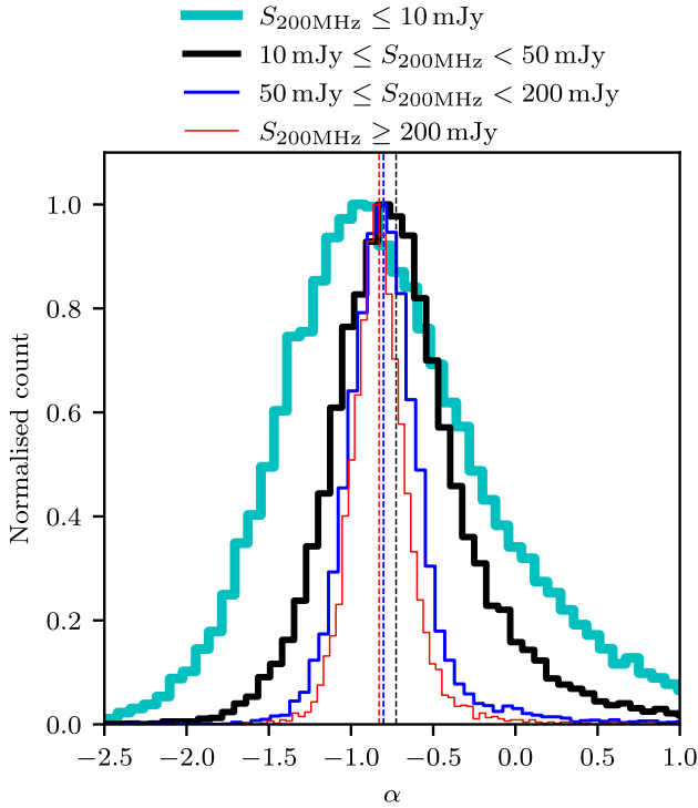
Figure 19. The spectral index distribution calculated for sources where the fit was successful (reduced \chi^2 < 1.93 ). The cyan line shows sources with S_{200\text{MHz}} < 10 mJy, the black line shows sources with 10 \leq S_{200\text{MHz}} < 50 mJy, the blue line shows sources with 50 \leq S_{200\text{MHz}} < 200 mJy, and the red line shows sources with S_{200\text{MHz}} \geq 200 mJy. The dashed vertical lines of the same colours show the median values for each flux density cut: -0.81 , -0.73 , -0.80 , and -0.83 , respectively.
