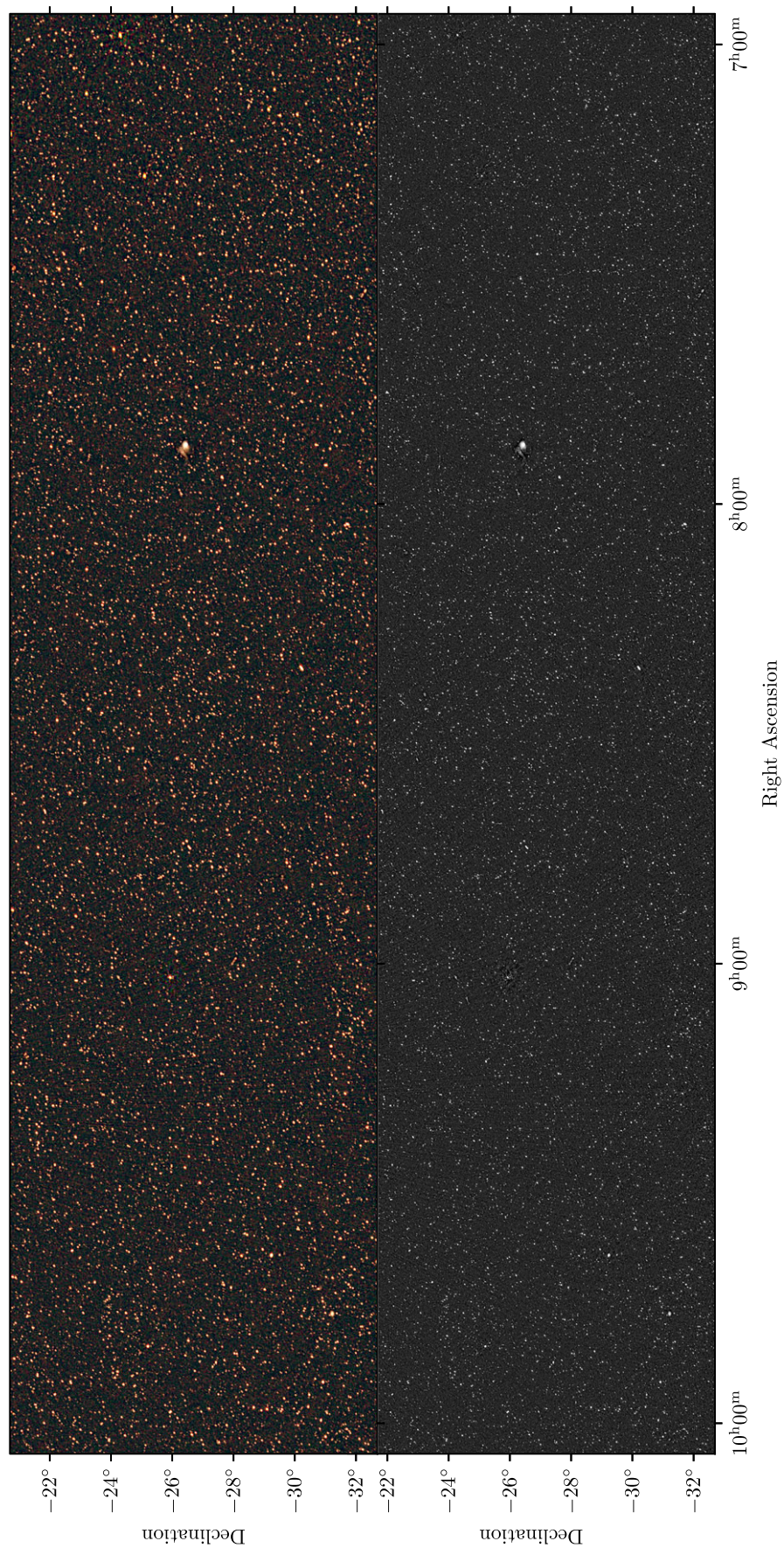
Figure 6. Continuum mosaics from this data release, for RA 7–10 h. Figure formatting is identical to Figure 5.
