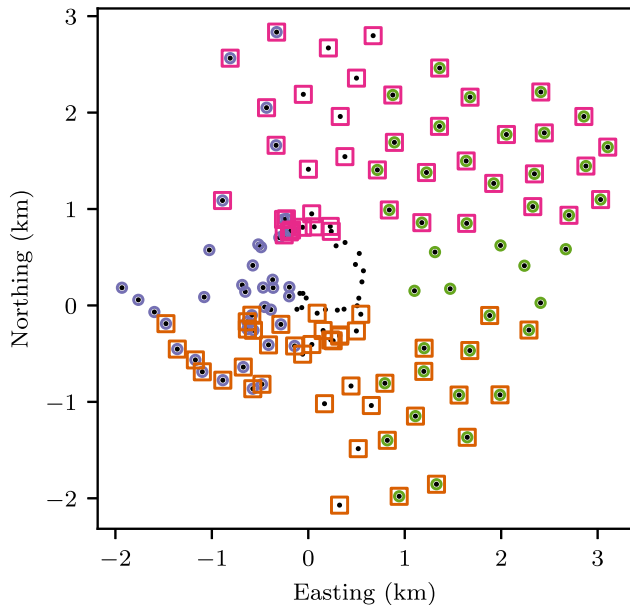
Figure 21. The layout of the tiles comprising the MWA Phase II extended configuration, overlaid with symbols representing sub-arrays used for ionospheric binocular imaging (Section 5.2). Pink and orange squares show the North and South pair, while green and lavender circles indicate the East and West pair.
