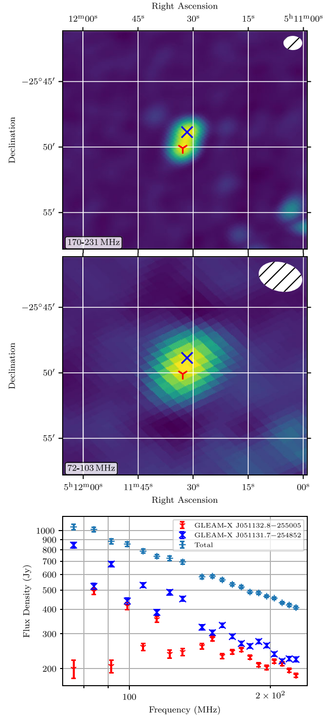
Figure 20. An example where the AEGEAN prioritised fitting routine was unable to produce consistent flux density measurements across sub-bands for a pair of components (GLEAM-X J051132.8 – 255005 and GLEAM-X J051131.7 – 254852) belonging to a single island. The top and middle panels are the 170–231 MHz and 72–103 MHz images towards these components, respectively, and the white ellipse in the upper right corner is the corresponding PSF. The bottom panel contains the SEDs of the individual components and their total.
