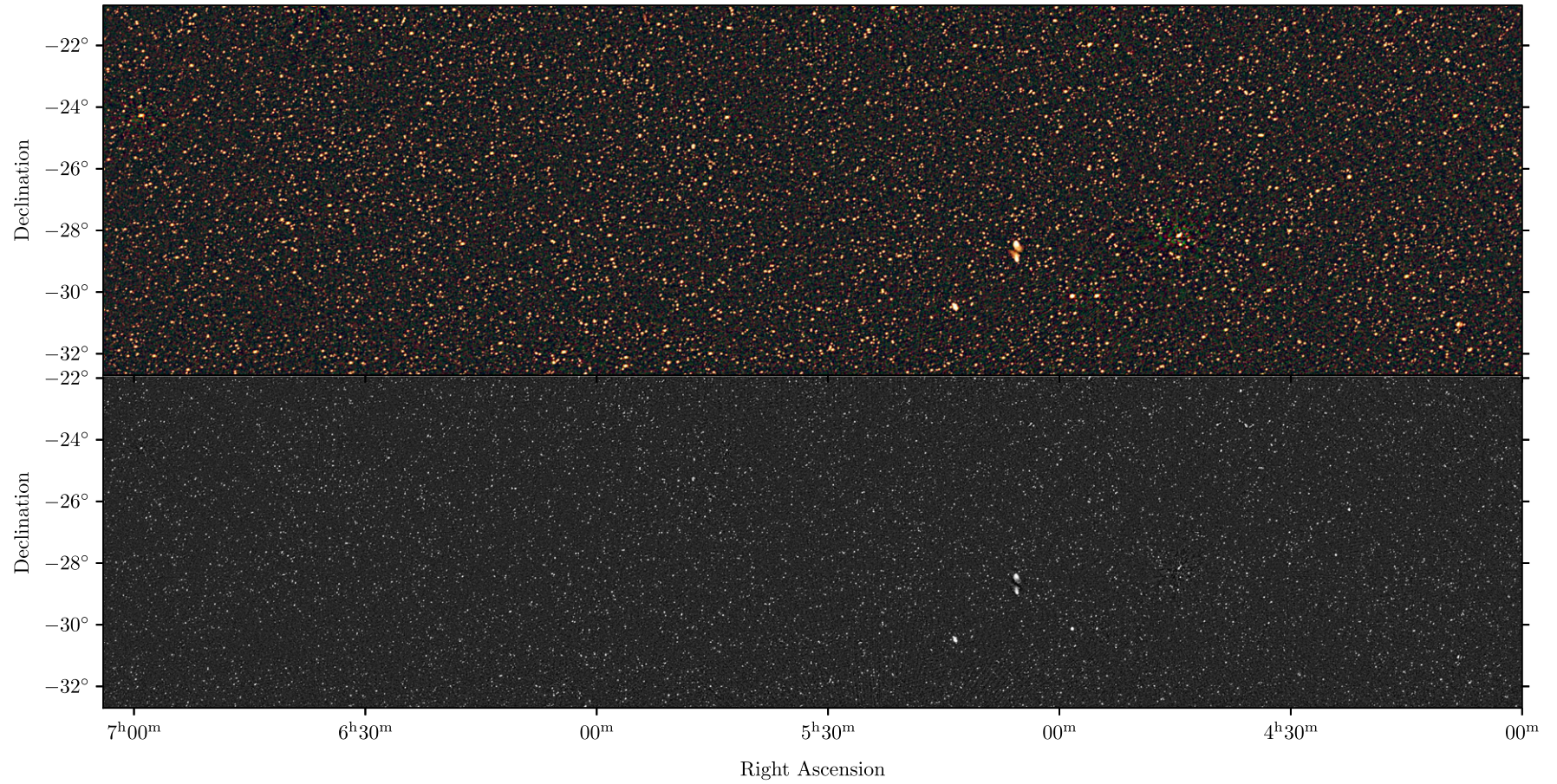
Figure 5. Continuum mosaics from this data release, for RA 4–7 h. In each sub-panel, the top image shows the 72–103 MHz (R), 103–134 MHz (G), and 139–170 MHz (B) data as an RGB cube, with an arcsinh stretch spanning -9 – 200 mJy beam ^{-1} ; the lower image shows the 170–231 MHz source-finding image, with an arcsinh stretch spanning -3 – 200 mJy beam ^{-1} .
