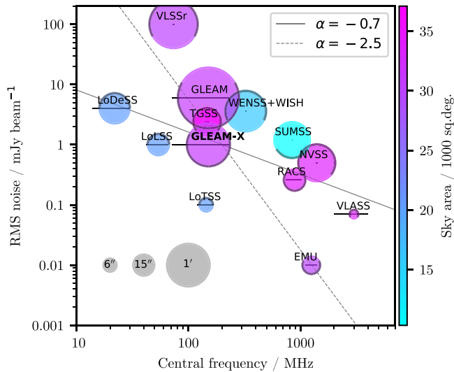
Figure 1. Summary of the sensitivity, frequency, resolution, and sky coverage of a selection of recent and planned large-area radio surveys. The size of the markers is proportional to the survey resolution (full-width-half-maximum of the restoring beam; examples shown in the lower left corner) and their colours show the sky coverage planned. The darkened edges of each marker show the Declination coverage of each survey. The width of each horizontal line shows the frequency range covered by that survey. Representative solid ( \alpha = -0.7 ) and dashed ( \alpha = -2.5 ) lines show the expected brightness at different frequencies for sources of brightness 1 \text{ mJy beam}^{-1} at 200 MHz.
