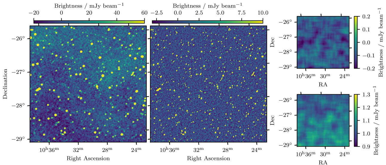
Figure 8. Ten sq. deg. of the wideband source-finding mosaic centred on RA 10^{\text{h}}30^{\text{m}} Dec -27^{\circ}30' ; the left panel shows the image from GLEAM ExGal; the middle panel shows the image from this work; the top and bottom right panels show, respectively, the background and RMS noise of the GLEAM-X data as measured by BANE. GLEAM ExGal contains 212 components in this region, and the average RMS noise is 6 \text{ mJy beam}^{-1} ; GLEAM-X contains 548 components and the average RMS noise is 1.1 \text{ mJy beam}^{-1} .
