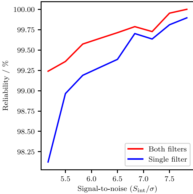
Figure 17. Estimates of the reliability of the catalogue as a function of signal to noise. The lower blue curve shows a conservative estimate without filtering negative sources detected on the edges of positive sources. The upper red curve shows a more generous estimate derived after filtering these sources out. In comparison, GLEAM ExGal has a reliability of 98.9%–99.8% at these signal-to-noise levels.
