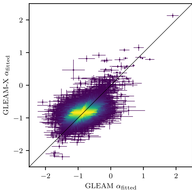
Figure 10. Spectral indices \alpha from the spectra fitted across the 20 7.68-MHz narrow bands of GLEAM-X (ordinate) against GLEAM (abscissa), for compact sources matched between the two surveys in the region released in this work. The colour axis shows an arbitrary number density scaling to show where there are more points. The error bars are the fitting errors obtained for each source, dominated by the flux density calibration error at the bright end and the local RMS noise at the faint end. The diagonal line shows a 1:1 ratio.
