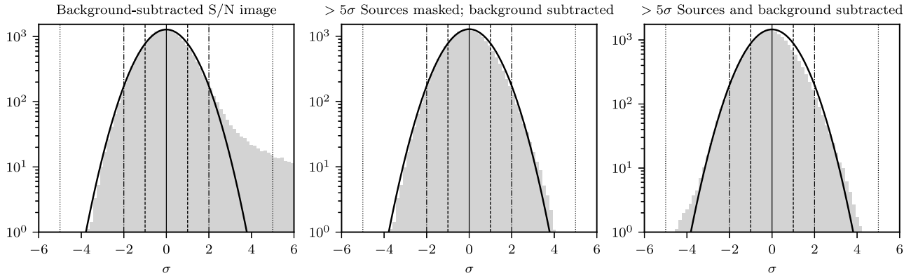
Figure 11. Noise distribution in a typical 18 square degrees of the wideband source-finding image. BANE measures the average RMS in this region to be 1.06 \text{ mJy beam}^{-1} . To more clearly show any deviation from Gaussian noise, the ordinate is plotted on a log scale. The leftmost panel shows the distribution of the S/Ns of the pixels in the image produced by subtracting the background and dividing by the RMS map measured by BANE; the right panel shows the S/N distribution after masking all sources detected at 5\sigma down to 0.2\sigma . The light grey histograms show the data. The black lines show Gaussians with \sigma = 1 ; vertical solid lines indicate the mean values. |S/N| = 1\sigma is shown with dashed lines, |S/N| = 2\sigma is shown with dash-dotted lines, and |S/N| = 5\sigma is shown with dotted lines.
