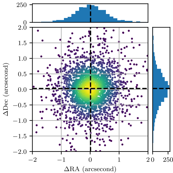
Figure 12. The astrometric offsets of 19771 isolated, compact, >50\sigma sources after cross-matching against the NVSS and SUMSS reference catalogue described in Section 4.2.3. Vertical and horizontal dashed lines indicate the mean offset values in the RA and Dec directions, respectively. Similarly, the horizontal and vertical histograms highlight the counts of the astrometry offsets in each direction.
