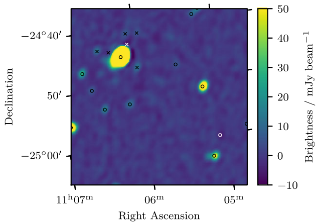
Figure 15. An example of filtering artefacts that present as spurious positive and negative sources around very bright sources. Black circles indicate detected positive components that are not filtered, while black \times s show positive components that are filtered. The white circle shows a negative source that was not filtered, while the white \times shows a negative source that was filtered for being too close to a bright source.
