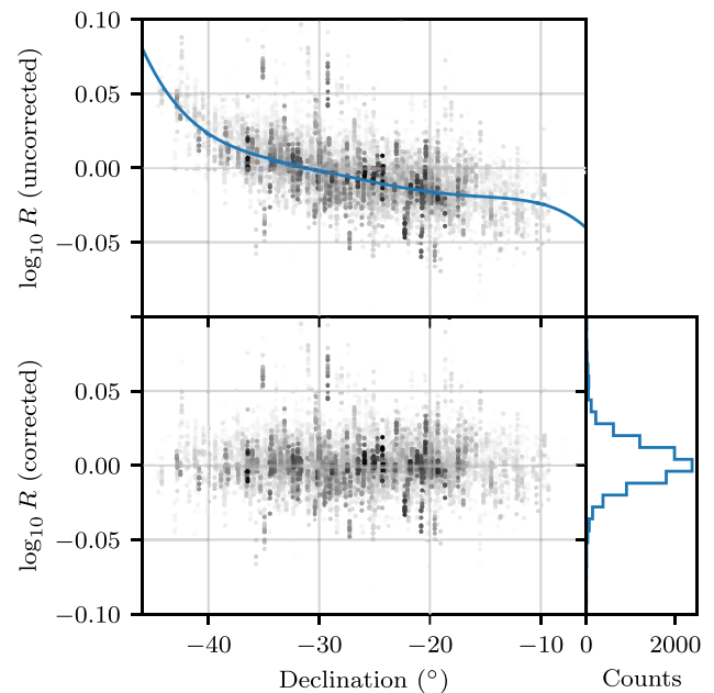
Figure 4. The accumulated flux density scale distribution across the snapshot images at 147–155 MHz from observations performed on 2018 February 20. The upper panel shows the change in \log_{10} R as a function of Dec, where R is the ratio of measured integrated flux density to model integrated flux density. The lower panel shows the same after the polynomial correction function (blue line) has been fit and applied. The adjacent histogram shows the resulting distribution of \log_{10} R over the drift scan. The full-width-at-half-maximum of the resulting histogram is \sim 2.5\% . Similar results are obtained for other frequency bands.
