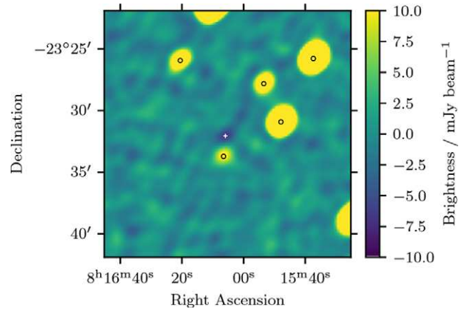
Figure 16. An example of a negative source found next to a positive source that could optionally be filtered when generating the reliability estimate. Black circles indicate detected positive components that are not filtered; the white + shows a negative source that can optionally be filtered.
