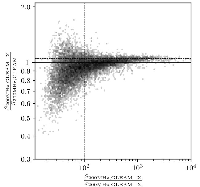
Figure 9. The ratio of the 200-MHz integrated flux densities measured in GLEAM-X and GLEAM, as a function of signal-to-noise in GLEAM-X, for compact sources matched between the two surveys in the region released in this work. The horizontal black line shows a ratio of 1 and the horizontal dashed black line shows a ratio of 1.05, which is a better visual fit at high signal-to-noise. The vertical line is plotted at a signal-to-noise of 100, approximately the 90% completeness level of GLEAM in this region. The error bars are omitted for clarity, but as the quadrature sum of the measurement errors in both surveys, increase to ~10% at the 90% completeness limit of GLEAM, and to ~30% at the faintest levels.
