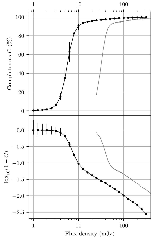
Figure 13. Completeness as a function of integrated flux density at 200 MHz for the region published in this work, which has RMS noise 1.27 \pm 0.15 \text{ mJy beam}^{-1} . The top panel shows the completeness C ; to better display the completeness as it approaches 100%, the bottom panel shows \log_{10}(1 - C) . Black markers and lines indicate GLEAM-X; for comparison, grey markers and lines show the completeness of GLEAM for a low-noise region used to determine source counts in GLEAM ExGal ( \sim 2500 \text{ deg}^2 with RMS noise 6.8 \pm 1.3 \text{ mJy beam}^{-1} ).
