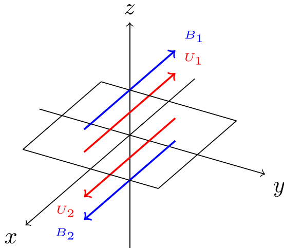
FIG. 1. An illustration of the coordinate system. The two uniform magnetic fields \mathbf{B}_1 and \mathbf{B}_2 are aligned along the stream velocity, and their directions can be either parallel or anti-parallel. We will show that the EKHI depends only on the square of the magnetic field and is independent of their directions.
