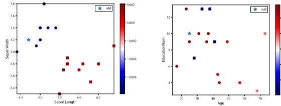
(a) Iris. (b) Adult. Fig. 2: Changes of Shapley value.
