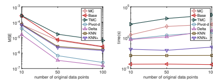
(a) MSEs. (b) Time cost.
