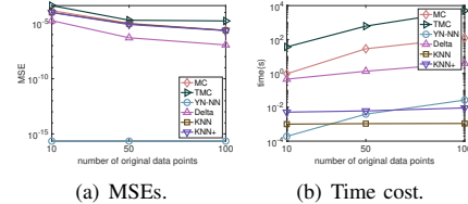
Fig. 5: Deleting a data point.
