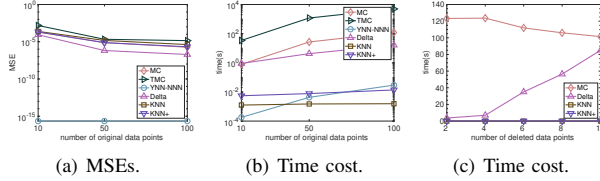
Fig. 6: Deleting multiple data points.
