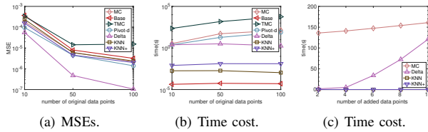
Fig. 4: Adding multiple data points.
