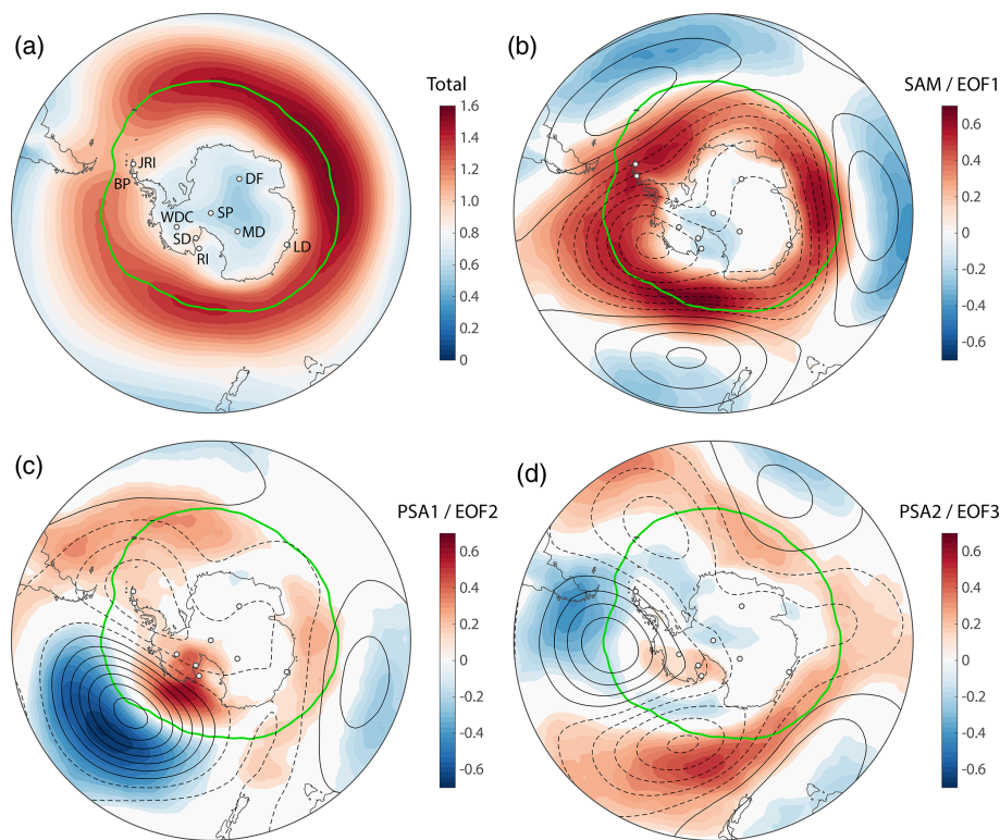
Figure 5. Modes of SH extratropical atmospheric variability and their link to synoptic-scale surface pressure variability in Antarctica. (a) Annual mean \Phi in units of percent per day ( \% \text{ d}^{-1} ). (b) Colors show correlation between \Phi and the southern annular mode (SAM) index, with the 500 hPa geopotential height anomalies superimposed in 10 m contours (positive contours solid, negative contours dashed). (c) As panel (b) , but for the Pacific–South American Pattern 1 (PSA1). (d) As panel (b) , but for the Pacific–South American Pattern 2 (PSA2). SAM, PSA1, and PSA2 are defined as the first, second, and third EOFs (empirical orthogonal functions), respectively, of the 500 hPa geopotential height anomalies in 20–90° S monthly values in the 1979–2017 ERA-Interim reanalysis (Dee et al., 2011). In all panels the latitude of maximum \Phi is denoted by the green line.
