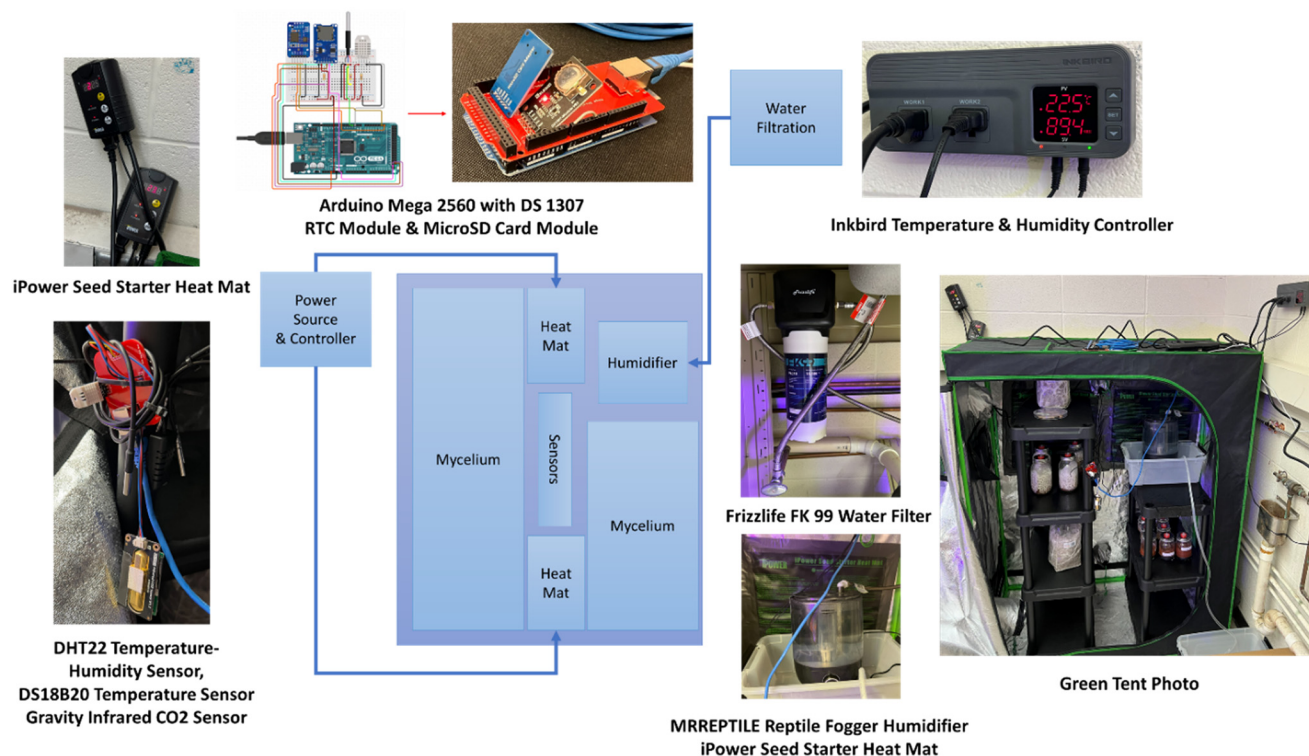
Fig. 1 Green tent appearance, a schematic of Arduino connection, a 3D circuit board, a placement chart of the system overview.
