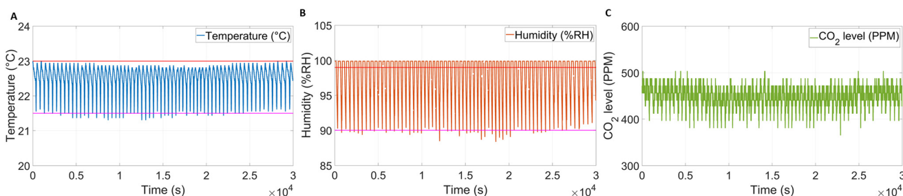
Fig. 4 The plot of the (A) temperature, (B) humidity, and (C) CO 2 history for the consequent 8 hours.
