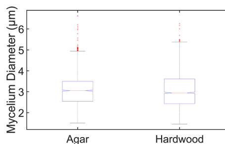
Fig. 6 Distribution of two groups data (diameter of mycelium fiber on agar versus wood surface), the ANOVA test suggests that the mycelium diameters of the two groups are equivalent.
