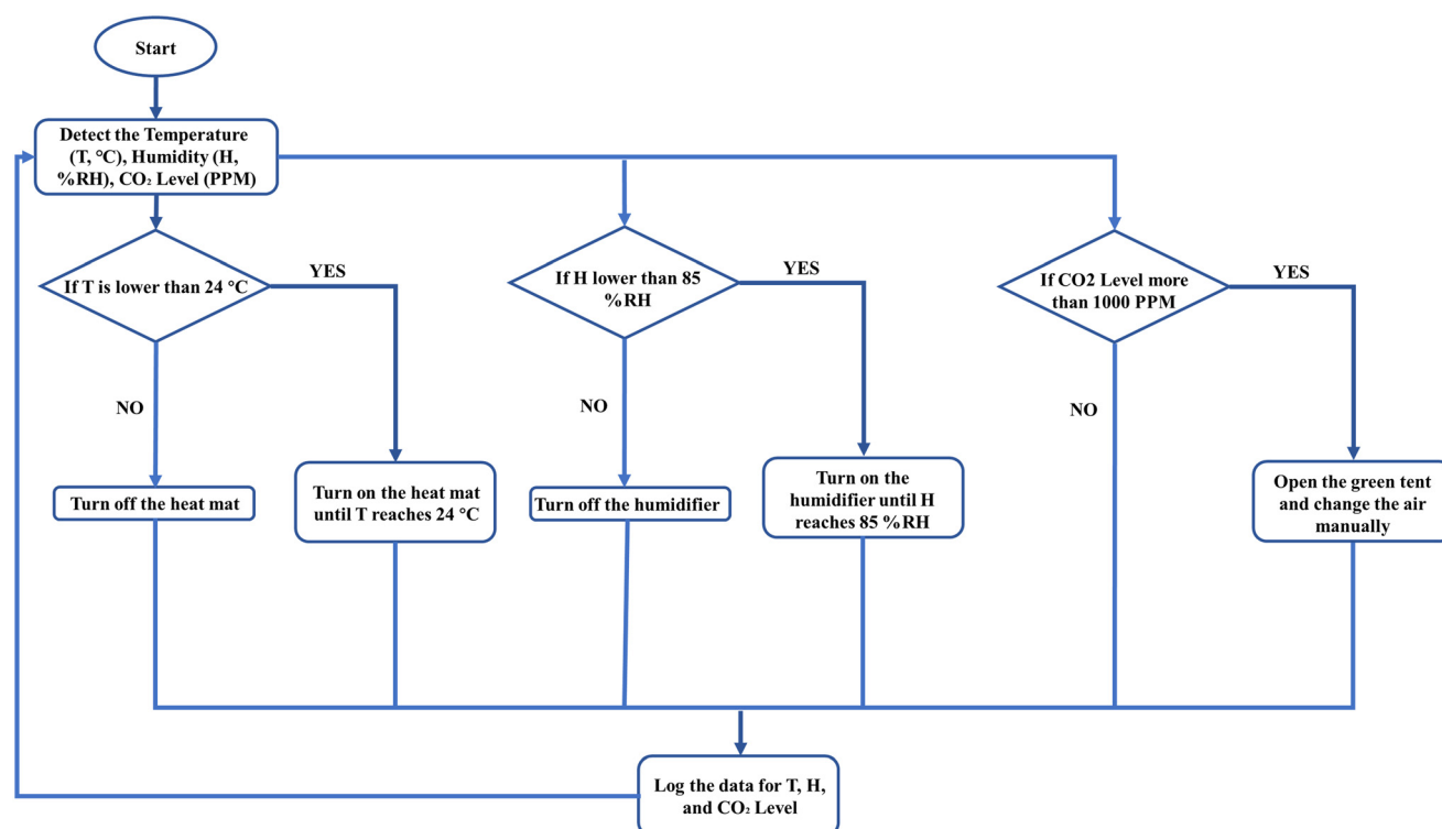
Fig. 2 A schematic information flow chart from the sensor to Arduino and controllers.
