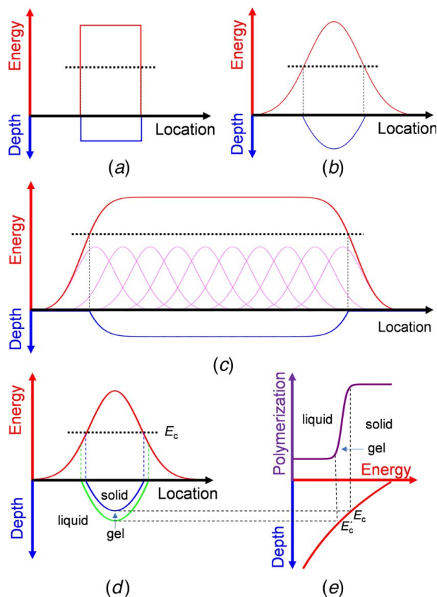
Fig. 1 PSL Photopolymerization simulation
