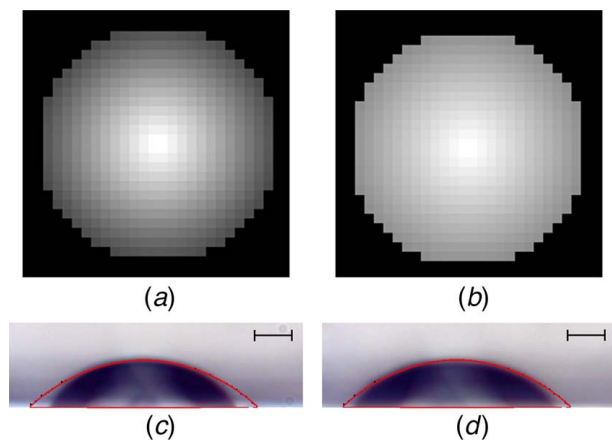
Fig. 16 (a) Grayscale 255–70, (b) grayscale 255–140, comparison between desired/simulated profile and actual part for (c) gradient grayscale 255–70 (d) gradient grayscale 255–140. Scale bar size of 50 \mu\text{m} .
