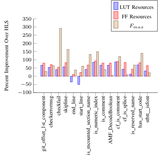
Figure 3. Differences in resource and time utilization. Higher bars show AUTOMATASYNTH using fewer resources and running at a higher frequency than HLS.
