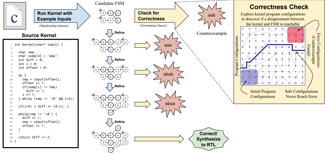
Figure 1. Example execution of AUTOMATASYNTH. The kernel function returns true for all strings within a hamming distance 2 of "aba". An initial automaton (triangles indicate starting states) is learned by running the kernel with example inputs. It is then checked for correctness using software verification to discover inputs that disagree. Four further refinements introduce new states and transitions through automated membership and termination queries. In this example, all counterexamples are strings the automaton should accept, but does not (false negatives). The final automaton passes all checks and is ready for synthesis to RTL.
