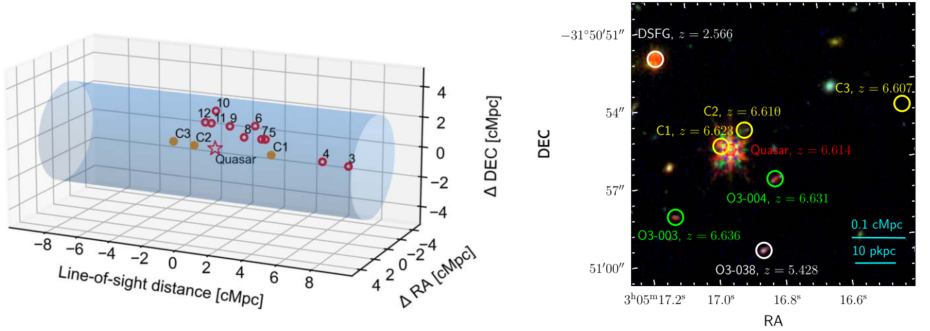
Figure 4. Left: 3D structure of the galaxy overdensity at z = 6.6 . In this panel, we show both [O III] and [C II] emitters in the vicinity of the quasar. The blue shaded region highlights a cylinder volume with a line-of-sight length of 2000 \text{ km s}^{-1} (or 18.8 \text{ cMpc} ) and a projected radius of 3.28 \text{ cMpc} at z = 6.6 (corresponding to an effective area of 5.5 \text{ arcmin}^2 in the projected plane). Right: immediate vicinity of quasar J0305–3150. The background is a RGB image made using NIRCcam imaging in F115W (B), F200W (G), and F356W (R). Quasar J0305–3150 is surrounded by three [C II] emitters (C1, C2, and C3; Venemans et al. 2019) and two [O III] emitters (ASPIRE-J0305M31-O3-003 and ASPIRE-J0305M31-O3-004) with line-of-sight velocities relative to the quasar of \Delta v_{\text{los}} < 1000 \text{ km s}^{-1} . Galaxy C3 is undetected in our deep JWST observations, which indicates that it is a DSFG. Galaxy [O III]-04 is also detected in Ly \alpha (Farina et al. 2017). Two foreground galaxies are also shown with a DSFG at z = 2.566 and a [O III] emitter at z = 5.428 .
