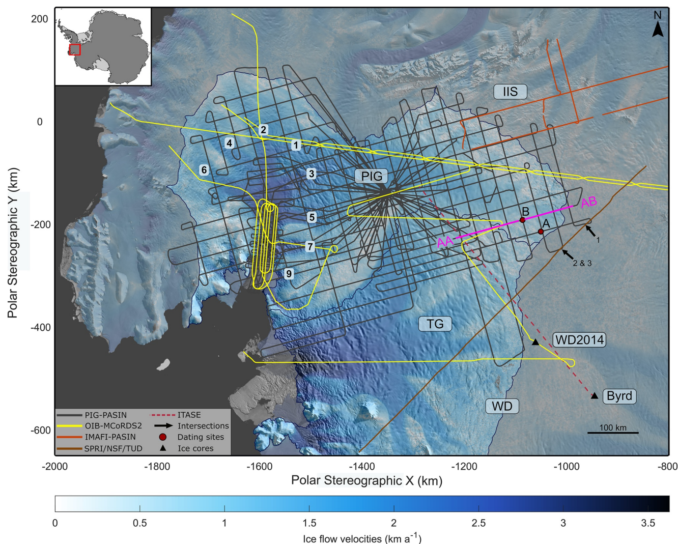
Figure 1. Map of study area with the data sets and key locations mentioned in this study. The inset in top left corner shows the region of interest (red box). Airborne survey lines included in this study: PIG-PASIN (gray), OIB-MCoRDS2 (yellow), IMAFI-PASIN transects flown over Institute Ice Stream (IIS) and intersecting the PIG catchment (orange), SPRI/NSF/TUD line (brown), overlaid on top of ice flow velocities from Rignot et al. (2017) and MODIS Mosaic of Antarctica (Scambos et al., 2007). Also included is the long, ITASE GPR-transect (dashed red) through which the 17.5 \pm 0.5 ka layer from Jacobel and Welch (2005) was traced. The numbers shown over PIG's trunk represent the eight fast-flowing tributaries (1–7, 9) mentioned in this study. The WAIS Divide (WD2014) and Byrd ice cores are represented by the two black triangles, and the black arrows represent the three intersections between the SPRI/NSF/TUD-traced IRHs and this study. The two red circles show the two sites (Sites A and B) where the 1-D age-depth model was used. The AA–AB segment (magenta) shows a subset of the control line where IRHs were first identified over PIG-PASIN (see Figure 2). The Western Divide is shown as WD on the map. The ICESat IMBIE basins of Pine Island Glacier (PIG) and Thwaites Glacier (TG) (Zwally et al., 2012) are annotated on the map and delimited by the blue outline lines.
