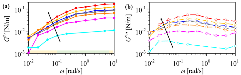
Fig. 4 Dynamic moduli at increasing surface pressure (shown by the arrow) of \Pi = 5, 10, 15, 20, 30, 40 , and 50 mN/m; a storage modulus, b loss modulus. Colored bars on horizontal axis depict the operating windows as follows: measured stress/inertia stress is (orange) < 5 , (yellow) > 5 , and (green) > 10
