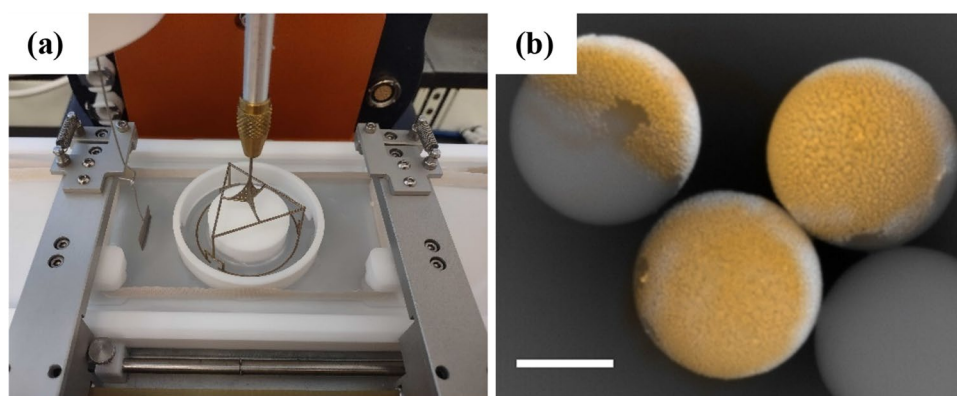
Fig. 1 a DWR geometry mounted in a Langmuir trough used to measure the shear rheology of Janus particle monolayers at the air–water interface. b Scanning electron microscope image of Janus particles with gold caps identified by the energy-dispersive X-ray spectroscopy analysis and colored in yellow. Scale bar is 500 nm
