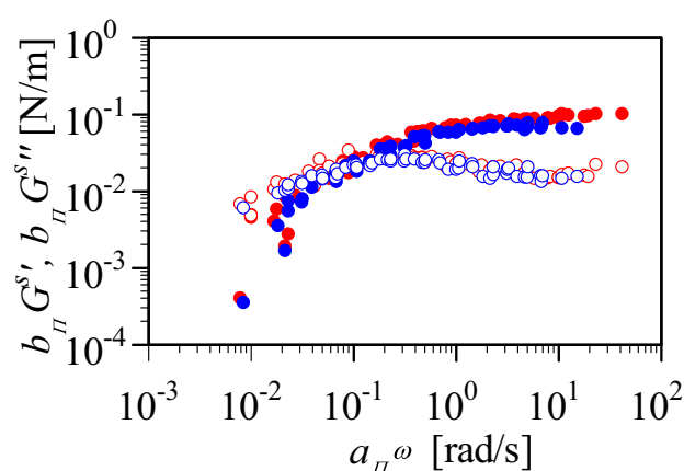
Fig. 10 Comparison of the master curves generated by the raw data and the subphase-corrected data obtained using the algorithm by Vandebriel et al. Red is the raw data and blue the corrected data
