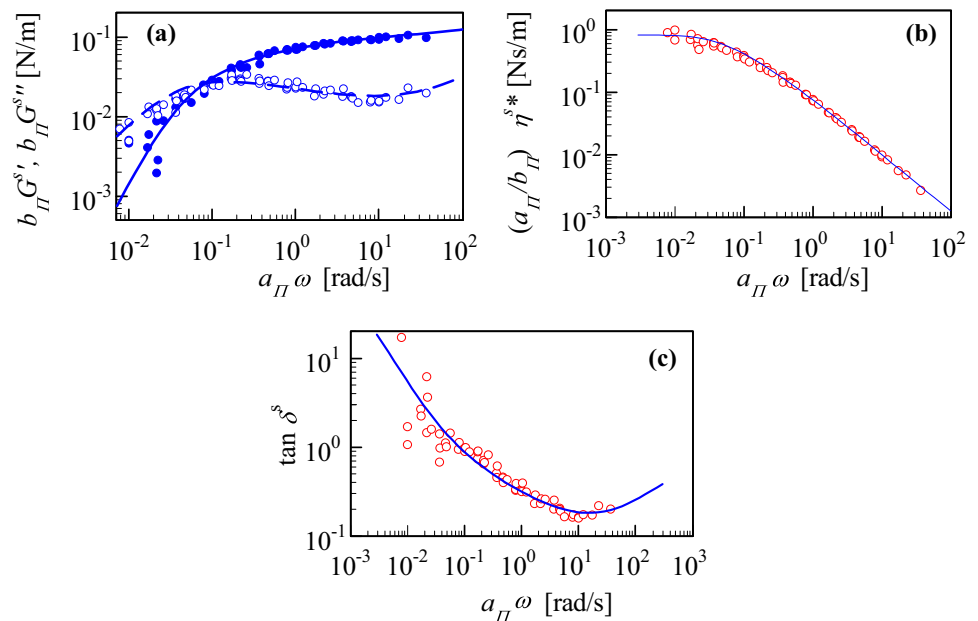
Fig. 6 a Dynamic modulus data merged onto \Pi = 30 mN/m; b_{\Pi} G^s(\omega) closed symbols, b_{\Pi} G^{s''}(\omega) open symbols. b Complex shear viscosity from master curve at \Pi = 30 mN/m. c \tan \delta^s for master curve with experimental data as red open circles. The lines belong to the power law relaxation time spectrum (Eq. 6), as discussed in the text, with parameters listed with Fig. 7
