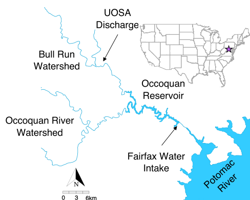
Figure 1. The Occoquan Reservoir is the nation’s first large-scale deliberate indirect potable reuse system for surface water augmentation. Inflow to the reservoir includes base flow and storm runoff from the Occoquan River and Bull Run watersheds, along with up to 54 million gallons per day of reclaimed water from the Upper Occoquan Service Authority (UOSA). Water from the Occoquan Reservoir is treated by Fairfax Water, the water wholesaler, and from there passes to various water distributors for up to 1 million drinking water customers in Northern Virginia.
