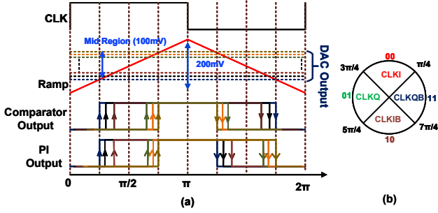
Fig. 4. (a) PI timing diagram for DIN<7:6>=00 , and (b) quadrant selection for the ramp signal input to the comparator using different DIN<7:6> .
