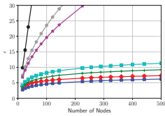
Fig. 5: \epsilon v.s. number of nodes ( \alpha = 0.5 ).
