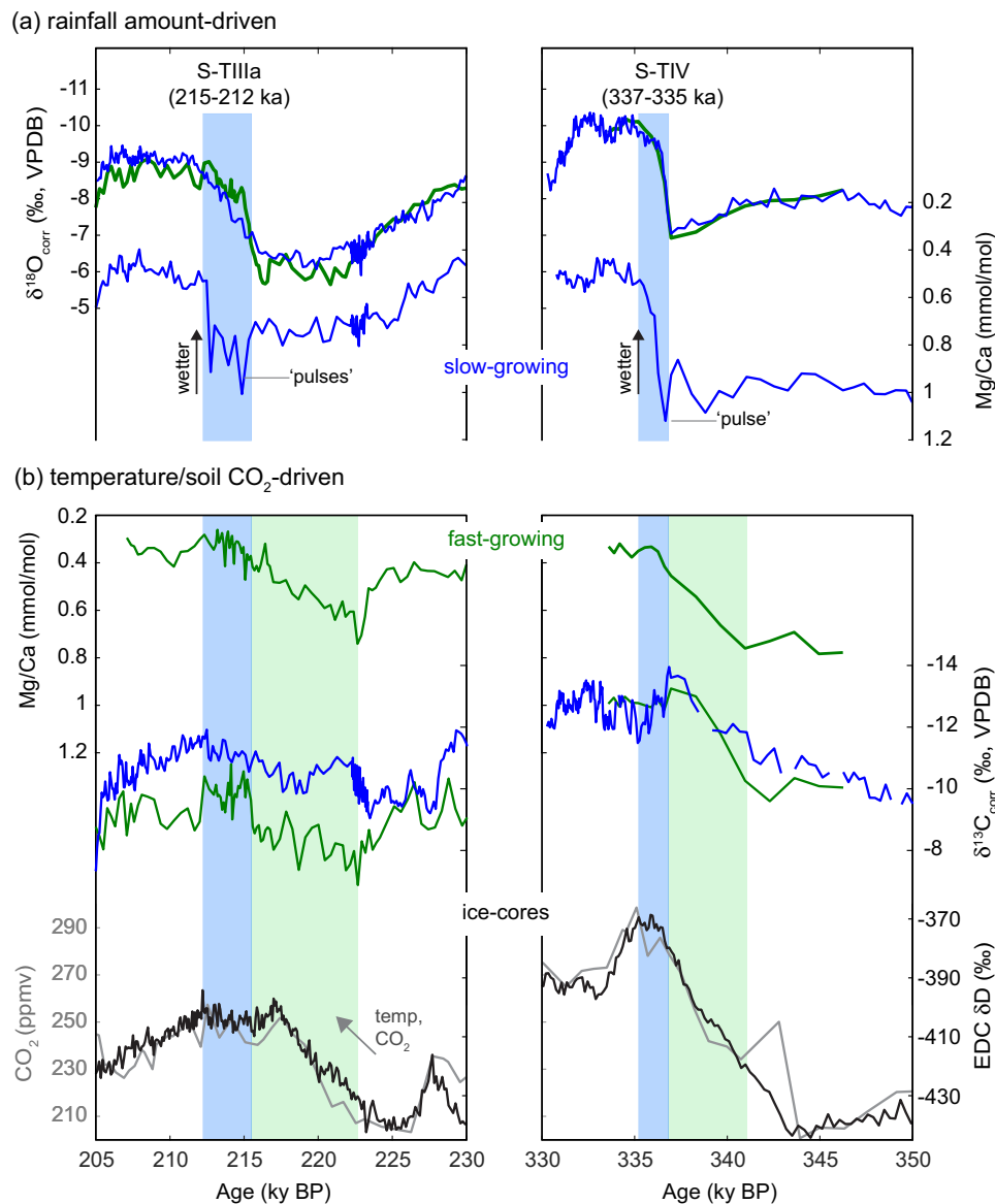
Fig. 5 Sulawesi stalagmite proxies driven by rainfall amount versus temperature and soil CO 2 . a Sulawesi stalagmite \delta^{18}O records (corrected for ice volume) and slow-growing stalagmite Mg/Ca. b Fast-growing Sulawesi stalagmite Mg/Ca and all stalagmite \delta^{13}C records compared with Vostok ice core measurements of atmospheric CO 2 (grey) and EPICA Dome C deuterium (black) plotted on the AICC chronology 59–61 (lower panel). The gradual trend in the fast-growing stalagmite Mg/Ca (green) corresponds with changes in stalagmite \delta^{13}C (corrected for atmospheric CO 2 effect), atmospheric CO 2 and global temperature/ \delta D (grey arrows). This Mg/Ca response is attributed to soil-karst processes, driven by vegetation changes (green bars). The step-change in the slow-growing stalagmite Mg/Ca (blue) corresponds with the deglacial transition in \delta^{18}O and is attributed to water-karst PCP processes driven by infiltration. Note the pulses during Sulawesi glacial terminations S-TIIla (215–212 ky BP) and S-TIV (337–335 ky BP), interpreted as a response to increased infiltration (see text for details). The durations of S-TIIla (215–212 ky BP) and S-TIV (337–335 ky BP) are based on all four stalagmite \delta^{18}O change points and coinciding change points in slow-growing stalagmite Mg/Ca (blue bars, Supplementary Fig. S5).
