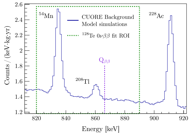
FIG. 1. \mathcal{M}_1 spectrum from the CUORE background model simulations in the proximity of the ^{128}\text{Te} 0\nu\beta\beta decay Q_{\beta\beta} . From left to right: ^{54}\text{Mn} \gamma (834.8 keV), ^{208}\text{Tl} \gamma (860.6 keV), and ^{228}\text{Ac} \gamma (911.2 keV). The ROI for this analysis is denoted by the dashed green box, and includes the ^{54}\text{Mn} and ^{208}\text{Tl} lines.
