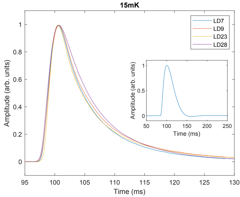
Figure 4. Normalized mean pulses of four LDs measured at the optimum working point (corresponding to a high NTD bias, at a few nA current) with a detector plate temperature of 15 mK. Inset: mean pulse of a LD at low NTD bias (0.1 nA corresponding to 80 \text{ M}\Omega of the NTD resistance) which shows a comparatively slow signal with a bouncing pulse shape.
