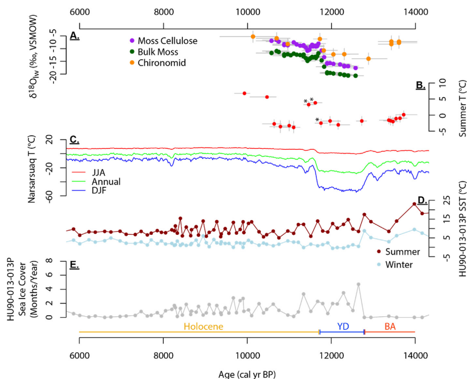
Fig. 6. Lake N14 records compared to regional climate records from ~14,000–6000 cal yr BP. (A) Lake water \delta^{18}\text{O} ( \delta^{18}\text{O}_{\text{lw}} ) modeled from \delta^{18}\text{O} values of moss cellulose, bulk moss, and chironomid head capsules at Lake N14. Points represent midpoint age of each sample. Vertical gray lines include analytical uncertainty and uncertainty from regression equations for converting to \delta^{18}\text{O}_{\text{lw}} . Uncertainties are smaller than the plotted points for moss and cellulose data. Horizontal gray lines reflect age uncertainty in the model associated with the uppermost and lowermost sediment depths of each sample. (B) Chironomid assemblage-based summer air temperature from Lake N14 (via WA-PLS modeling; Medeiros et al., 2022). Starred samples had <50 identified head capsules due to low concentrations. In some cases, uncertainty is smaller than the size of points. (C) Seasonally resolved modeled temperatures from Narsarsuaq to the southern tip of Greenland (Buizert et al., 2018). (D) Seasonally resolved sea surface temperatures from core HU90-013–013P off the coast of south Greenland (Solignac et al., 2004; de Vernal and Hillaire Marcel, 2006). (E) Months of sea ice cover per year (with 50% sea ice concentration or greater) based on core HU90-013–013P (gray). Basal colored bars indicate the approximate timing of the Holocene (yellow), Younger Dryas (YD; blue), and Bølling-Allerød (BA; red) based on the chronology in Rasmussen et al. (2006). (For interpretation of the references to color in this figure legend, the reader is referred to the Web version of this article.)
