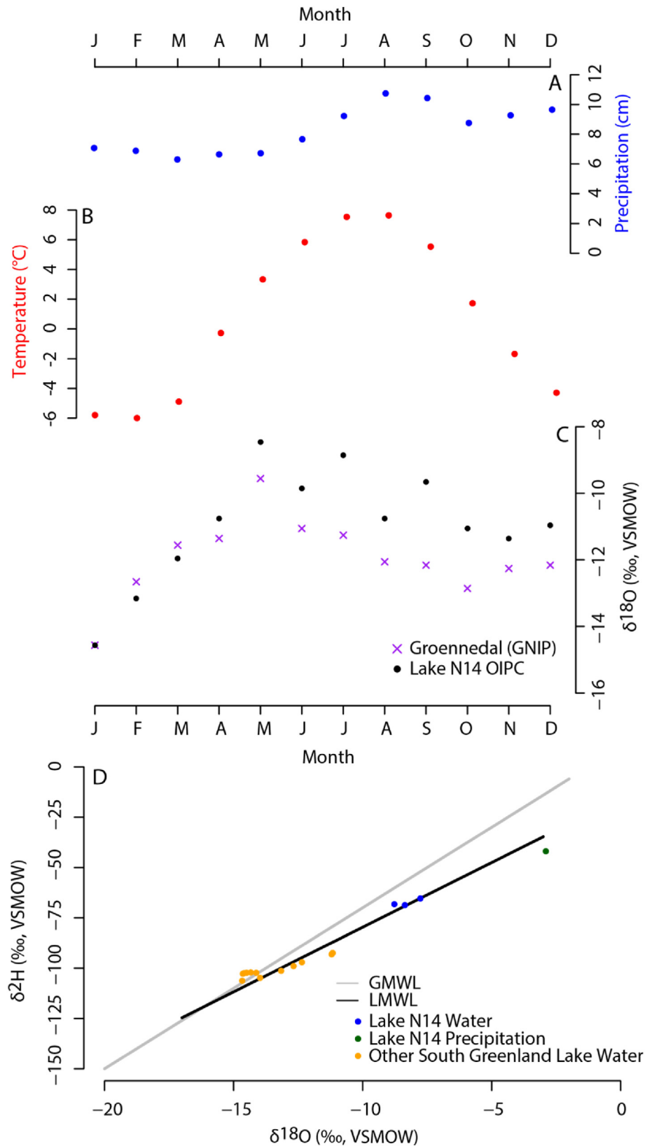
Fig. 2. Monthly precipitation amount (A) and temperature (B) from the Qaortoq weather station (Cappelen, 2019) alongside monthly precipitation isotope measurements (C) from the Groennedal station (IAEA/WMO, 2015) and modeled monthly precipitation isotopes from the Online Isotopes in Precipitation Calculator (Bowen, 2022; Bowen et al., 2005; IAEA/WMO, 2015). (D) The global meteoric water line (GMWL) and local meteoric water line (LMWL; based on data from the Groennedal GNIP station (IAEA/WMO, 2015)) are plotted alongside measured values of Lake N14 lake water and precipitation, and measured values from other south Greenland lakes sampled in the Summer of 2016 (Lasher and Axford, 2019).
