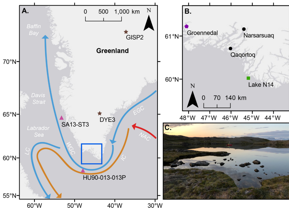
Fig. 1. (A) An overview of Greenland with key ocean currents (NAC=North Atlantic Current, EGC = East Greenland Current, IC=Irminger Current, WGC=West Greenland Current, LC = Labrador Current). Brown stars indicate locations of the GISP2 (72°58.2'N, 38°48.0'W) and DYE3 (65°10.8'N, 43°49.2'W) ice core sites. Pink triangles indicate the locations of marine sediment cores HU90-013-013P (58°12.59'N, 48°22.40'W) and SA13-ST3 (64°26.74'N, 52°47.64'W). Blue box indicates the extent of panel B. (B) The setting of Lake N14 (green square) in southernmost Greenland. Also shown are the towns of Qaqortoq and Narsarsuaq (black dots) and the Groennedal Global Networks of Isotopes in Precipitation (GNIP) station (purple pentagon). (C) Lake N14 in August 2019. Photo taken by Peter Puleo. (For interpretation of the references to color in this figure legend, the reader is referred to the Web version of this article.)
