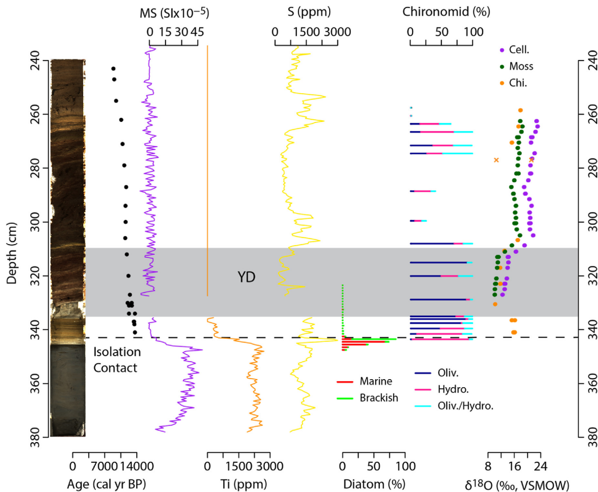
Fig. 4. Core 19-N14-N7 visual stratigraphy, bulk sediment composition, biotic assemblages, and \delta^{18}\text{O} of aquatic organic materials. Both y-axes show total sediment depth (cm). From left to right, the data presented includes a core image, calibrated ^{14}\text{C} ages (black dots), bulk sediment magnetic susceptibility (MS; purple), titanium (orange), and sulfur (yellow) in bulk sediments, relative abundances of marine and brackish indicator diatom taxa, relative abundances of extreme-cold indicator chironomid taxa (Oliv. = Oliveridia , Hydro. = Hydrobaenus ), and \delta^{18}\text{O} of aquatic moss cellulose (cell.), bulk moss (moss), and subfossil chironomid head capsules (chi.). The two orange xs are outlier duplicate \delta^{18}\text{O} samples that were removed. The analytical uncertainty of the \delta^{18}\text{O} measurements is 0.4‰ and is smaller than the size of the points. Note that elemental concentrations are estimated in ppm but given instrument calibration uncertainties are most useful for relative comparisons. The approximate timing of the YD (based on Lake N14 \delta^{18}\text{O} values and supported by ^{14}\text{C} ages) is represented by the horizontal gray band. The black dashed line indicates the diatom inferred isolation contact. (For interpretation of the references to color in this figure legend, the reader is referred to the Web version of this article.)
