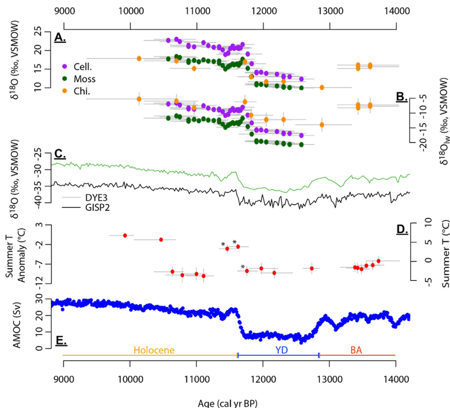
Fig. 5. Local and regional paleoclimate records from ~14,000–9000 cal yr BP. (A) Organic material \delta^{18}\text{O} values of moss cellulose (purple), bulk moss (green), and chironomid head capsules (orange) from Lake N14 sediment. (B) Lake water \delta^{18}\text{O} ( \delta^{18}\text{O}_{\text{lw}} ) modeled from \delta^{18}\text{O} values of moss cellulose, bulk moss, and chironomid head capsules (see methods). The points represent the midpoint age of each sample. The vertical gray uncertainty lines include the analytical uncertainty associated with the \delta^{18}\text{O} measurement (for panels A and B) and the uncertainty associated with the regression equations for converting to lake water (for panel B; see methods). These error bars are smaller than the points for all data in panel A and moss and cellulose data in panel B. The horizontal gray lines reflect the age uncertainty in the model associated with the uppermost and lowermost sediment depths of each sample. (C) Ice core \delta^{18}\text{O} values from DYE3 (green; Dansgaard et al., 1982; Badgley et al., 2020) and GISP2 (black; Grootes and Stuiver, 1997; see Fig. 1A for locations). (D) Chironomid assemblage-based summer air temperature anomalies from Lake N14 (via WA-PLS modeling; Medeiros et al., 2022). Starred samples had <50 identified head capsules due to low concentrations. Anomalies were calculated relative to modern species assemblages in surface sediments. (E) Modeled AMOC strength (Sv; 10^6 \text{ m}^3 \text{ s}^{-1} ) required to bring TraCE-21 K simulations and ice core reconstructions into agreement (Buizert et al., 2018). The basal colored bars indicate the approximate timing of the Holocene (yellow), Younger Dryas (YD; blue), and Bølling-Allerød (BA; red) based on the GISP2 isotope excursions (Rasmussen et al., 2006). (For interpretation of the references to color in this figure legend, the reader is referred to the Web version of this article.)
