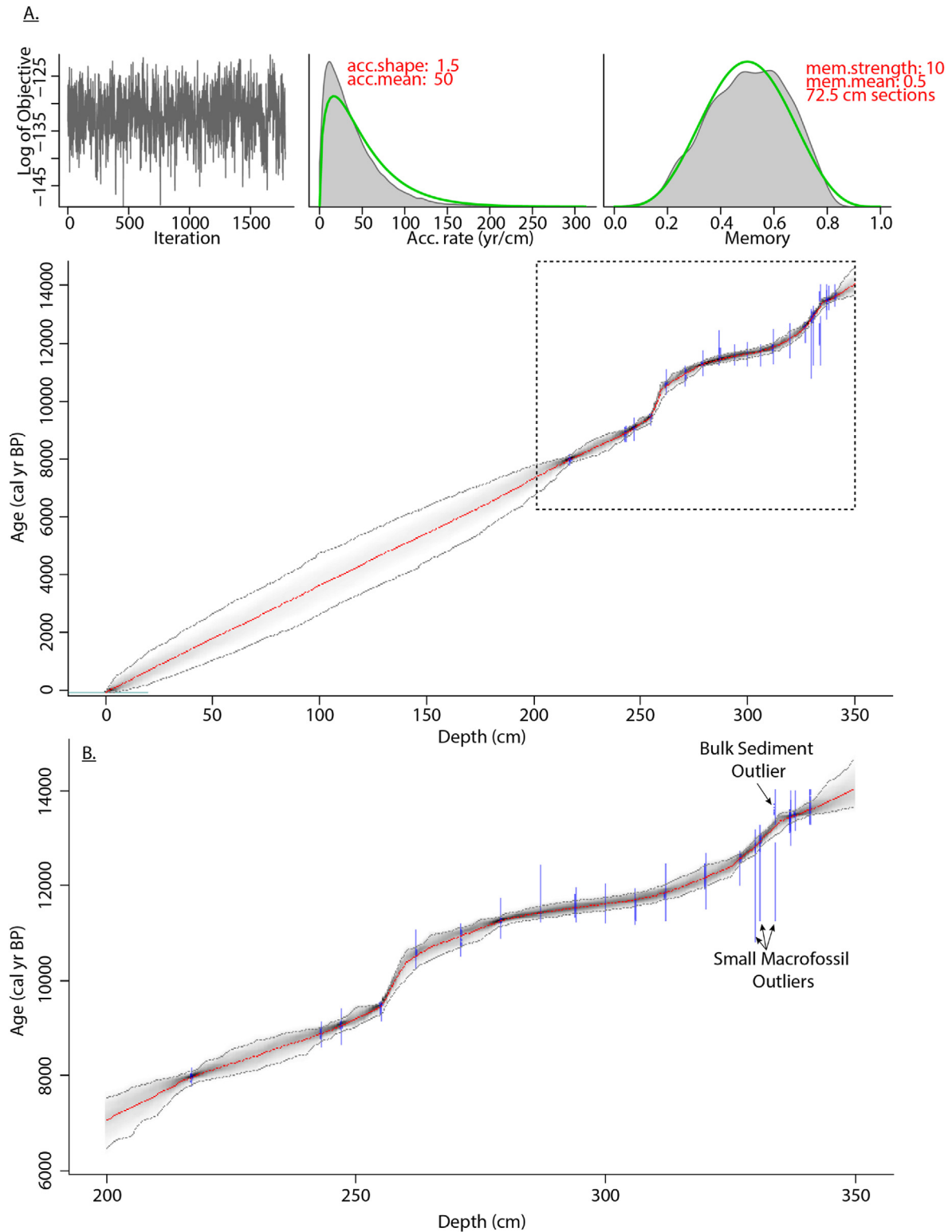
Fig. 3. (A) The full 19-N14-N7 age-depth model. The top three small figures (from left to right) show the Markov Chain Monte Carlo iterations, and the prior (green lines) and posterior densities (gray shaded areas) for the accumulation rate and memory. Below, blue shapes are the calibrated radiocarbon ages ( n = 24 ). The red line is the mean age. The edge of the gray cloud indicates the 95% confidence interval. Age model assumes -69 cal yr BP at 0 cm sediment depth. The dashed box in the age-depth model indicates the extent of panel B. (B) The lower portion of the 19-N14-N7 age-depth model (Medeiros et al., 2022). Arrows point to the outlier age-depth tie points discussed in the text. (For interpretation of the references to color in this figure legend, the reader is referred to the Web version of this article.)
