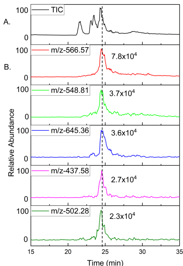
Fig. 4 A. TIC electropherogram for the six-protein CE separation. B. XIEs for the 5 most intense peptides that matched to carbonic anhydrase II. Each XIE is labelled with the m/z value. The maximum intensity is shown to the right of each XIE peak. The dotted black line highlights the consistency in the migration times of the peptides that stem from a given parent protein.
