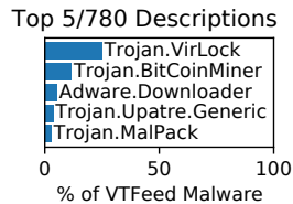
Figure 8: Distribution of malware descriptions for VTFeed given by Malwarebytes. Most prevalent is Trojan.VirLock at 25%.
