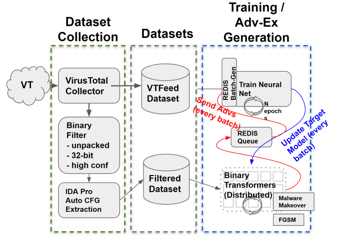
Figure 6: Distributed system for adversarially training DNNs.
