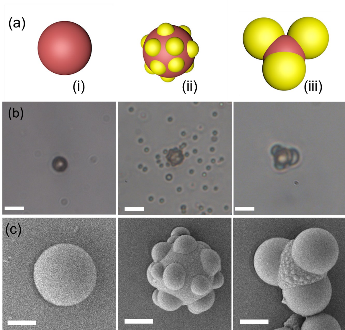
Fig. 2. Synthesis of three-lobed microrobots. (a) Scheme of synthesis (i) magnetic seed particles, (ii) heterogeneous nucleation of oil on the seeds, (iii) growth of droplets to achieve three lobes. (b) and (c) are corresponding respective optical and SEM images captured at different synthesis stages. Scale bars in (b) are 5 \mu\text{m} and in (c) are 2 \mu\text{m} .
