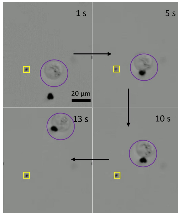
Fig. 7. Cell transportation by three-lobed microrobots. Time-lapse optical images of a microrobot transporting a cell. Yellow square is the reference point to mark a change in the position of cell being transported.
