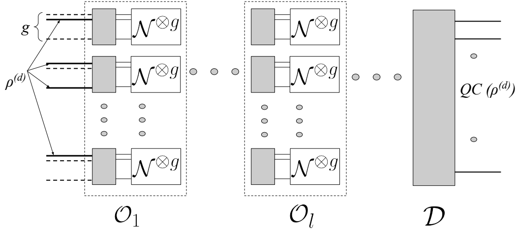
Figure 1: A schematic of the quantum computation model.
