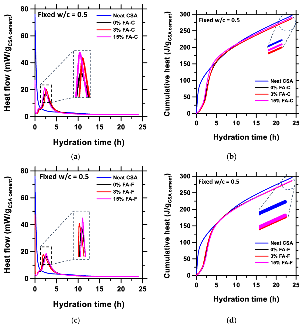
Figure 5. Isothermal calorimetry-based time-dependent (a) heat flow of [CSAC+FA-C] pastes, (b) cumulative heat released of [CSAC+FA-C] pastes, (c) heat flow of [CSAC+FA-F] pastes, (d) cumulative heat released of [CSAC+FA-F] pastes. “Neat CSA” represents paste with no added admixture. All pastes are for constant w/c = 0.5. Due to overlap of data points, some curves are shielded.
