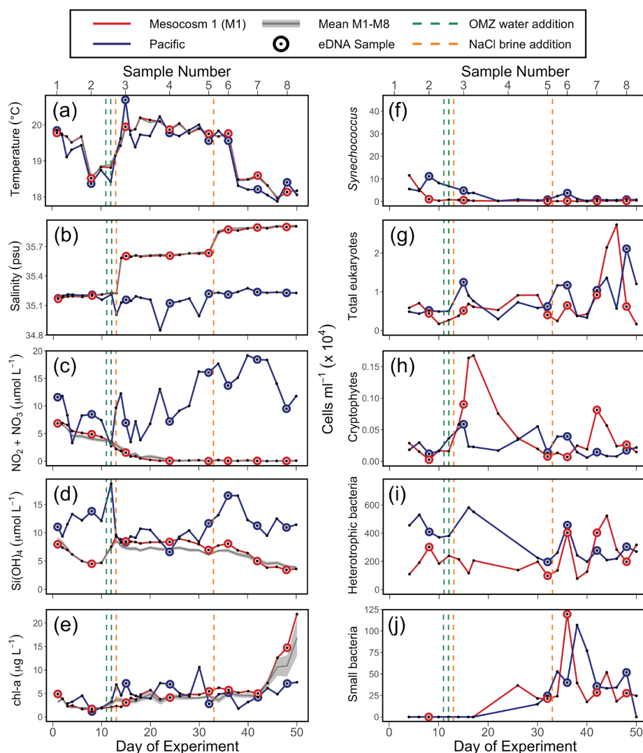
Figure 2. Physicochemical conditions, inorganic nutrients, and chlorophyll a (chl a ) in the mesocosms and unenclosed Pacific surface waters (a–e), with values averaged over the 0–17 m depth range. Flow cytometry results (f–j) from samples collected in the surface waters; these depths were 0–5 m on days 1 and 2, 0–10 m from day 3 to 28, and 0–12.5 m from day 29 to 50. For all panels, each individual sample is indicated. For (a), (b), (c), (d), and (e), the solid grey line represents the mean for all eight mesocosms; the shaded grey line is the mean \pm SE for all eight mesocosms. The green lines indicate exchange of \sim 20 \text{ m}^3 of OMZ water with water in the mesocosm (total volume \sim 50 \text{ m}^3 ) on days 11 and 12. The orange lines indicate NaCl brine additions on days 13 (69 L at a depth range of 10–17 m) and 33 (46 L at a depth range of 12.5–17 m). (a) Temperature. (b) Salinity. (c) \text{NO}_2^- + \text{NO}_3^- . (d) \text{Si(OH)}_4 . (e) Chlorophyll a (chl a ). (f) Synechococcus . (g) Photosynthetic eukaryotes. (h) Cryptophytes. (i) Heterotrophic (non-pigmented) bacteria. (j) Small bacteria (smaller than standard non-pigmented bacteria in the system).
