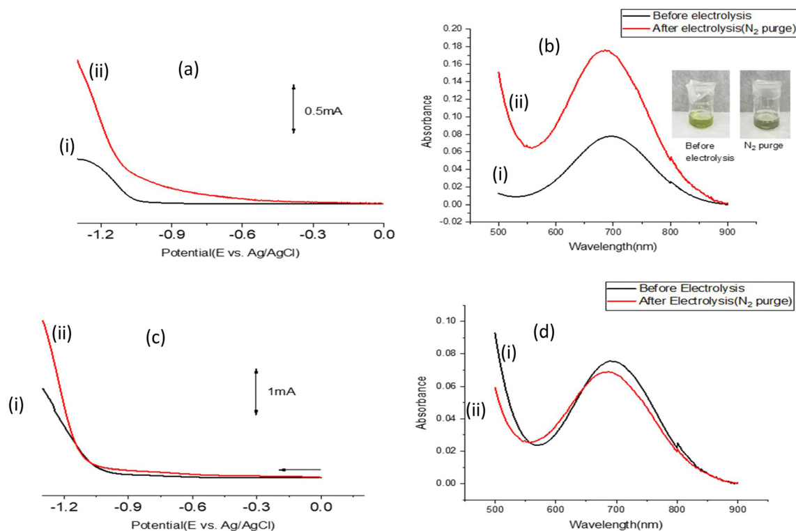
Fig. 3 (a) LSV curves of (i) bare FTO (black trace) and (ii) \text{TiO}_x\text{N}_y sample (red trace); (b) absorbance before and after electrolysis in \text{N}_2 environment in 0.1 M \text{Na}_2\text{SO}_4 solution at pH 1.6; (c) LSV curves of (i) bare FTO (black trace) and (ii) TiN sample (red trace); (d) corresponding absorbance before and after electrolysis in \text{N}_2 environment in 0.1 M \text{Na}_2\text{SO}_4 solution at pH 1.6.
