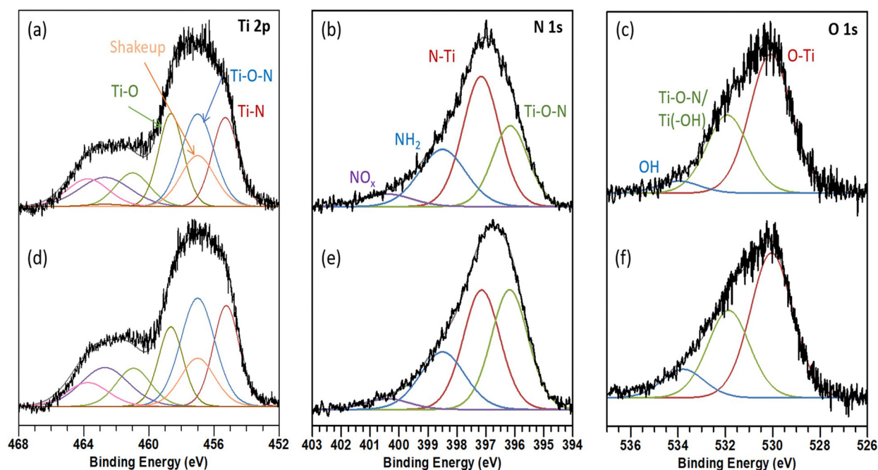
Fig. 2 XPS core level spectra after ambient exposure of (a–c) 'pure' TiN sample and (d–f) a TiO_xN_y sample. The XPS-derived N/O atomic ratio is \sim 1 for both films after ambient exposure.
