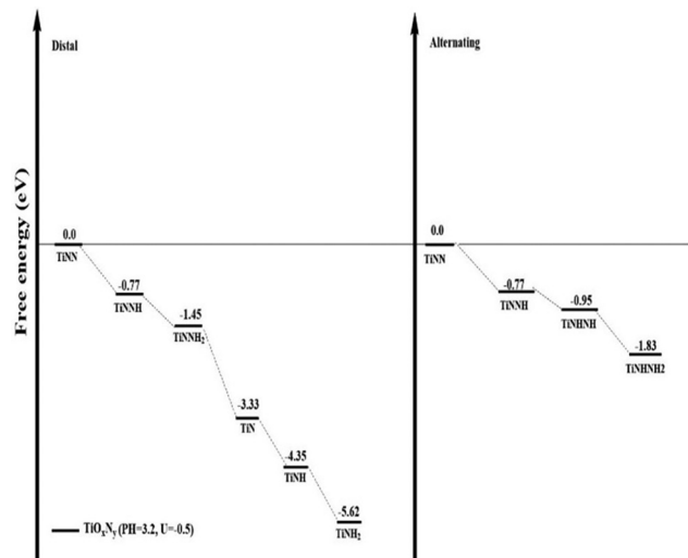
Fig. 12 N/H intermediate surface configurations for distal and alternating pathways in NRR for a Ti-oxynitride model. DFT-calculated relative energies (eV), E_{\text{rel}} , and assume pH = 3.2 and an applied potential of -0.5 V.
