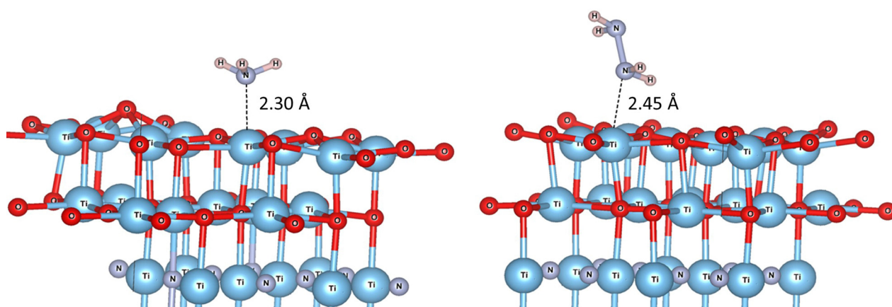
Fig. 14 Geometry optimization for rs- TiO_xN_y (001) does not result in hydrazine or ammonia being bonded to the surface.
