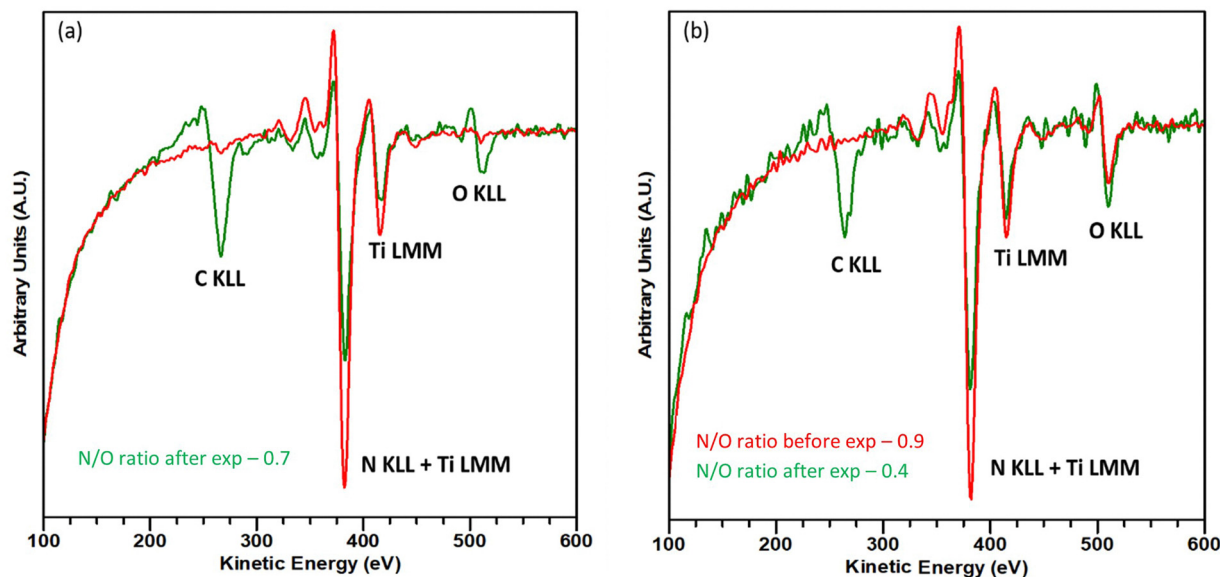
Fig. 1 In situ AES spectra after deposition and before ambient exposure (red trace) and also after 40 min ambient exposure (green trace) of (a) TiN sample; (b) TiON sample.
