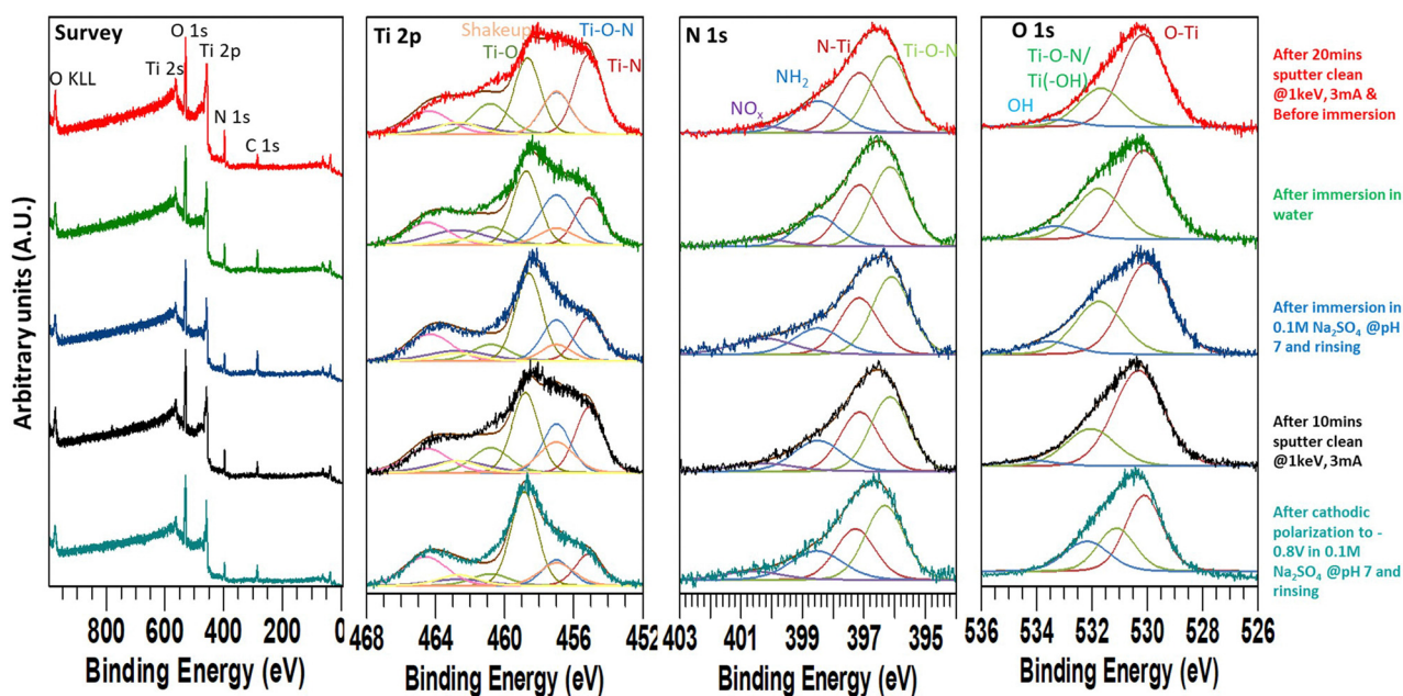
Fig. 11 XPS survey scan and core level spectra of a \text{TiO}_x\text{N}_y ( in situ AES N/O ratio \sim 1 ) sample for UHV-EC experiments at pH 7 in 0.1 M \text{Na}_2\text{SO}_4 solution.
