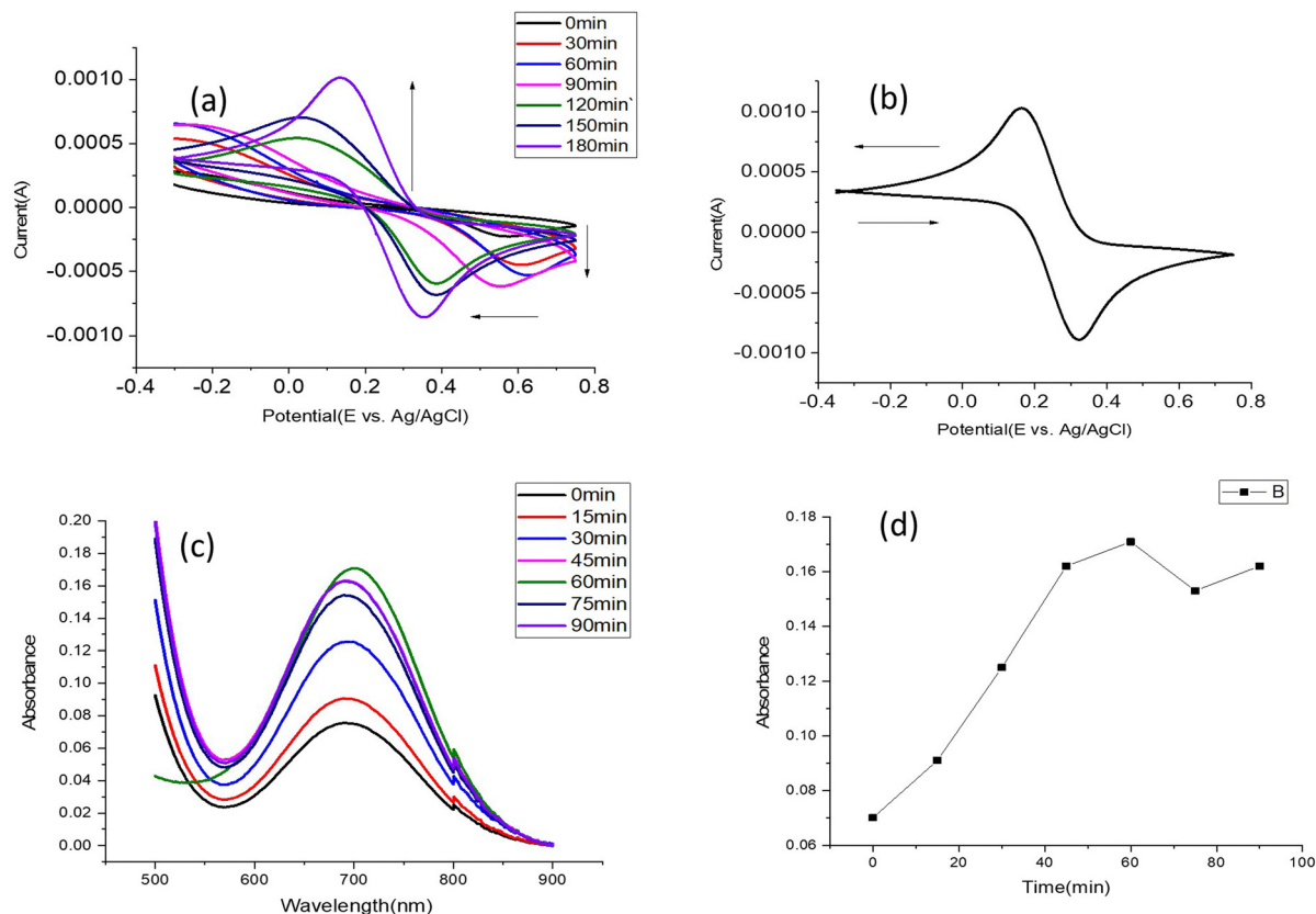
Fig. 8 (a) CVs of ferricyanide/ferrocyanide couple with TiON film before and at intervals during electrolysis for the evaluating the stability of the film at pH 3.2, and (b) CV of ferricyanide/ferrocyanide couple with bare FTO. (c) Absorbance spectra before and at intervals during electrolysis at -0.93 V vs. Ag/AgCl for the detection of \text{NH}_3 in \text{N}_2 environment in 0.1 M \text{Na}_2\text{SO}_4 solution at pH 3.2 (d) absorbance intensity/ \text{NH}_3 production vs. time based on the data in (c).
