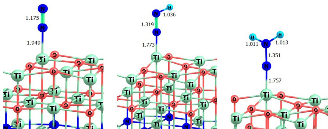
Fig. 13 DFT-optimized bond lengths for \text{TiO}_x\text{N}_y\text{-N}_2 , \text{TiO}_x\text{N}_y\text{-N}_2\text{H} , and \text{TiO}_x\text{N}_y\text{-N}_2\text{H}_2 surface models; bond lengths in Å.
