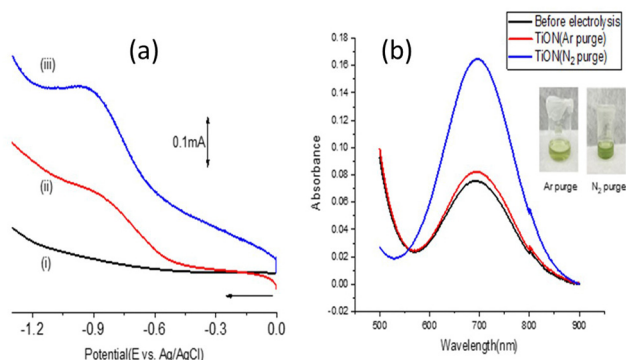
Fig. 4 (a) LSV curves for (i) bare FTO (ii) \text{TiO}_x\text{N}_y sample in Ar-environment (iii) \text{TiO}_x\text{N}_y sample in \text{N}_2 environment; (b) absorbance before and after electrolysis for the detection of ammonia in Ar & \text{N}_2 -environments.
