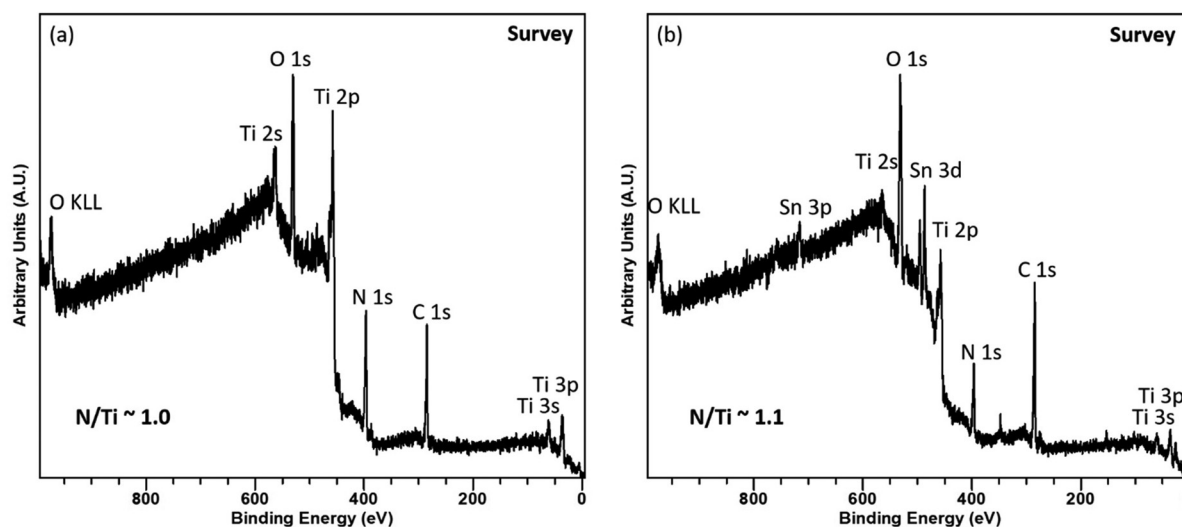
Fig. 7 Ex situ XPS survey scan of a TiON sample (a) before and (b) after 4.5 h multicyclic voltammograms at -0.93 V vs. Ag/AgCl in N_2 environment in 0.1 M Na_2SO_4 solution at pH 3.2.
