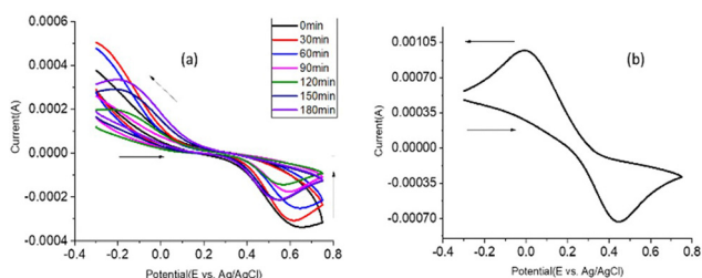
Fig. 9 (a) CV's of ferricyanide/ferrocyanide couple with TiON film before and at intervals during electrolysis for the evaluating the stability of the film at pH 7, and (b) CV of ferricyanide/ferrocyanide couple with bare FTO in 0.1 M \text{Na}_2\text{SO}_4 solution at pH 7.
