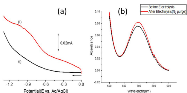
Fig. 5 (a) LSV curves of (i) bare FTO and (ii) TiN sample (b) absorbance before and after electrolysis for the detection of ammonia in \text{N}_2 environment in 0.1 M \text{Na}_2\text{SO}_4 solution at pH 3.2. In situ AES N/Ti \sim 1 before ambient exposure.
