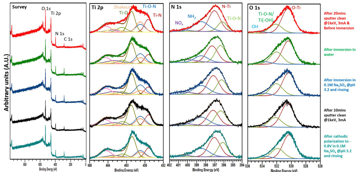
Fig. 10 XPS survey scan and core level spectra of a TiON ( in situ AES Ti/O/N ratio \sim 1 ) sample for UHV-EC experiments at pH 3.2 in 0.1 M \text{Na}_2\text{SO}_4 solution.
