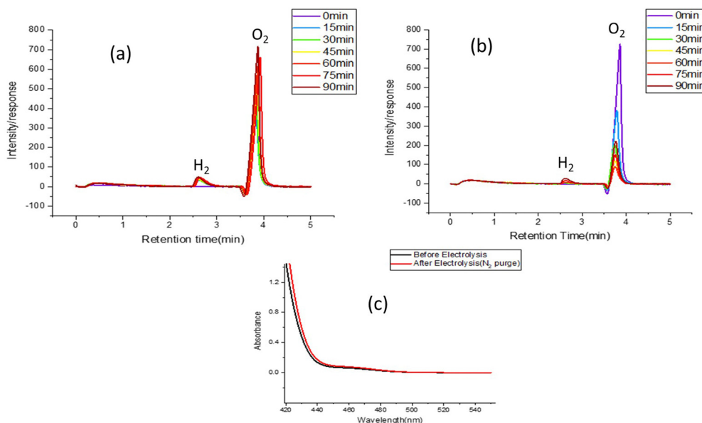
Fig. 6 Gas chromatogram of (a) bare FTO and (b) \text{TiO}_x\text{N}_y during electrolysis for the detection of \text{H}_2 in \text{N}_2 environment in 0.1 M \text{Na}_2\text{SO}_4 solution at pH 3.2 (c) absorbance before and after electrolysis for the detection of hydrazine in \text{N}_2 environment in 0.1 M \text{Na}_2\text{SO}_4 solution at pH 3.2.
