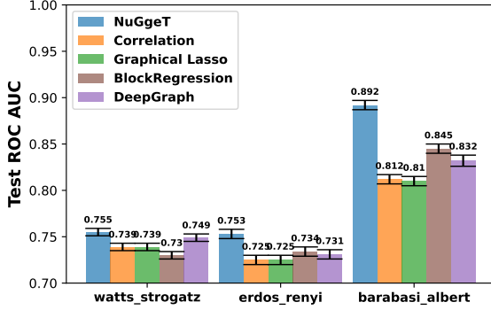
Figure 5. Results for BH graphical games.
