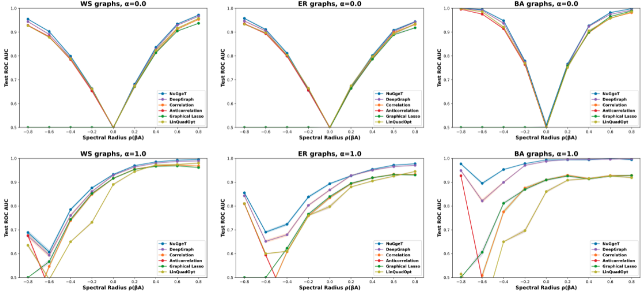
Figure 3. Results for linear quadratic games with varying \alpha and spectral radius \rho(\beta A) .
