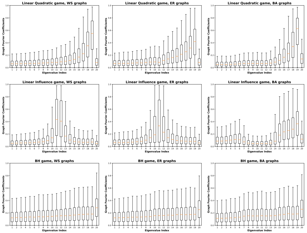
Figure 8. Magnitude of coefficients of normalised action vectors for different games and graphs. These are obtained by taking the Graph Fourier Transform of the actions, i.e., taking the inner product between the action and each of the adjacency matrix eigenvectors.
