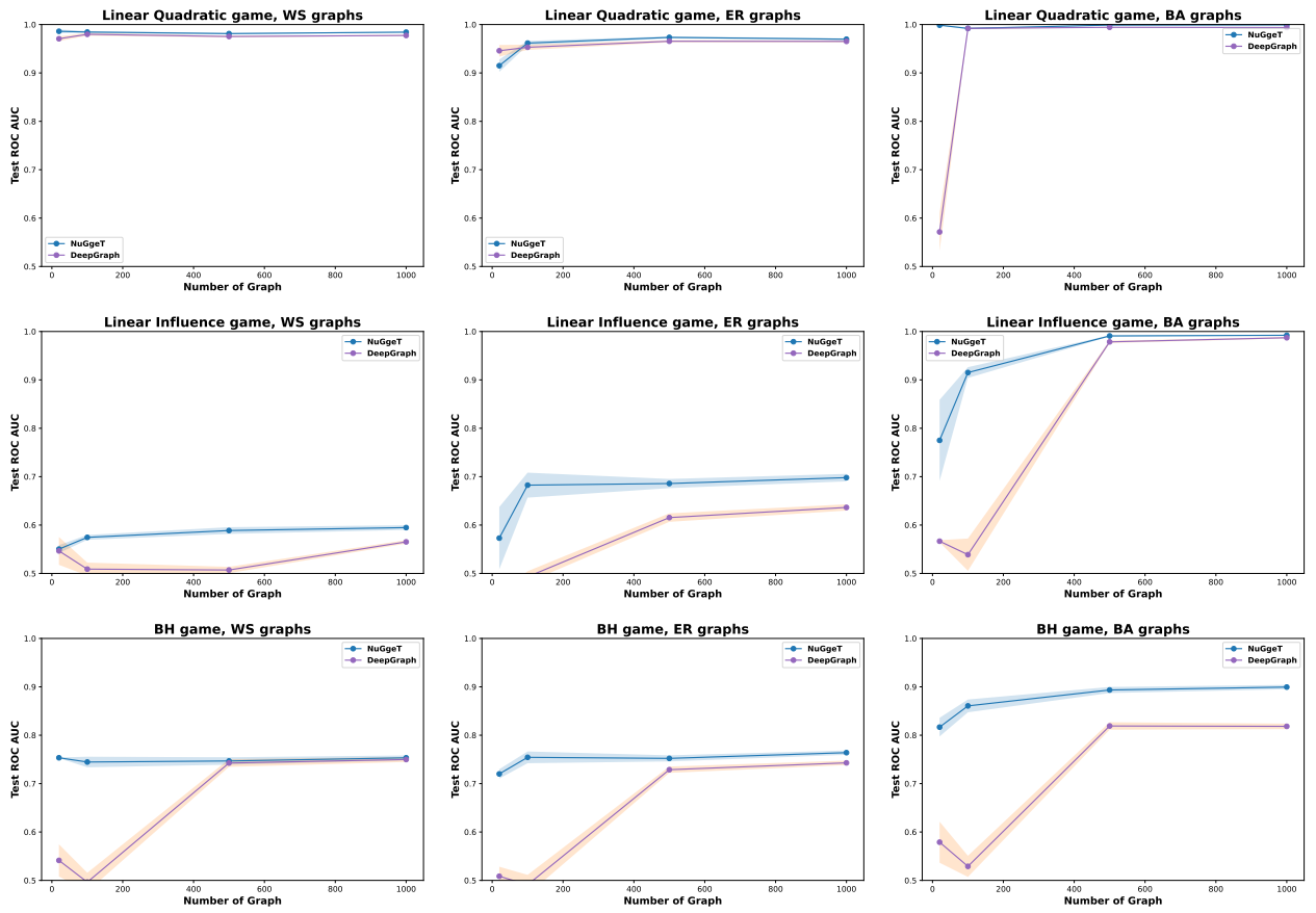
Figure 11. Results with varying number of training graphs.
