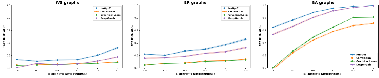
Figure 4. Results on linear influence games when varying the smoothness \alpha of the marginal benefits.
