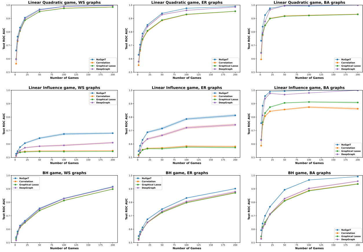
Figure 9. Results with varying number of games.
