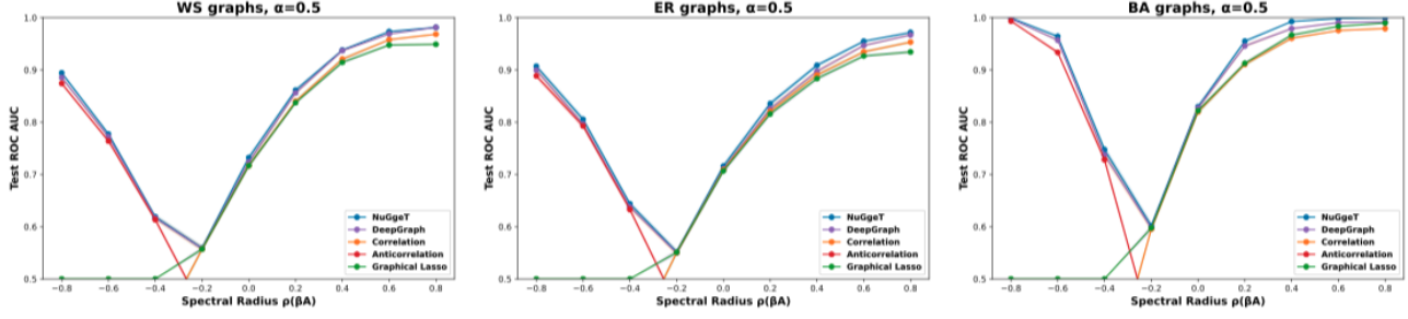
Figure 6. Results for linear quadratic games with \alpha = 0.5 and variable spectral radius \rho(\beta A) .
