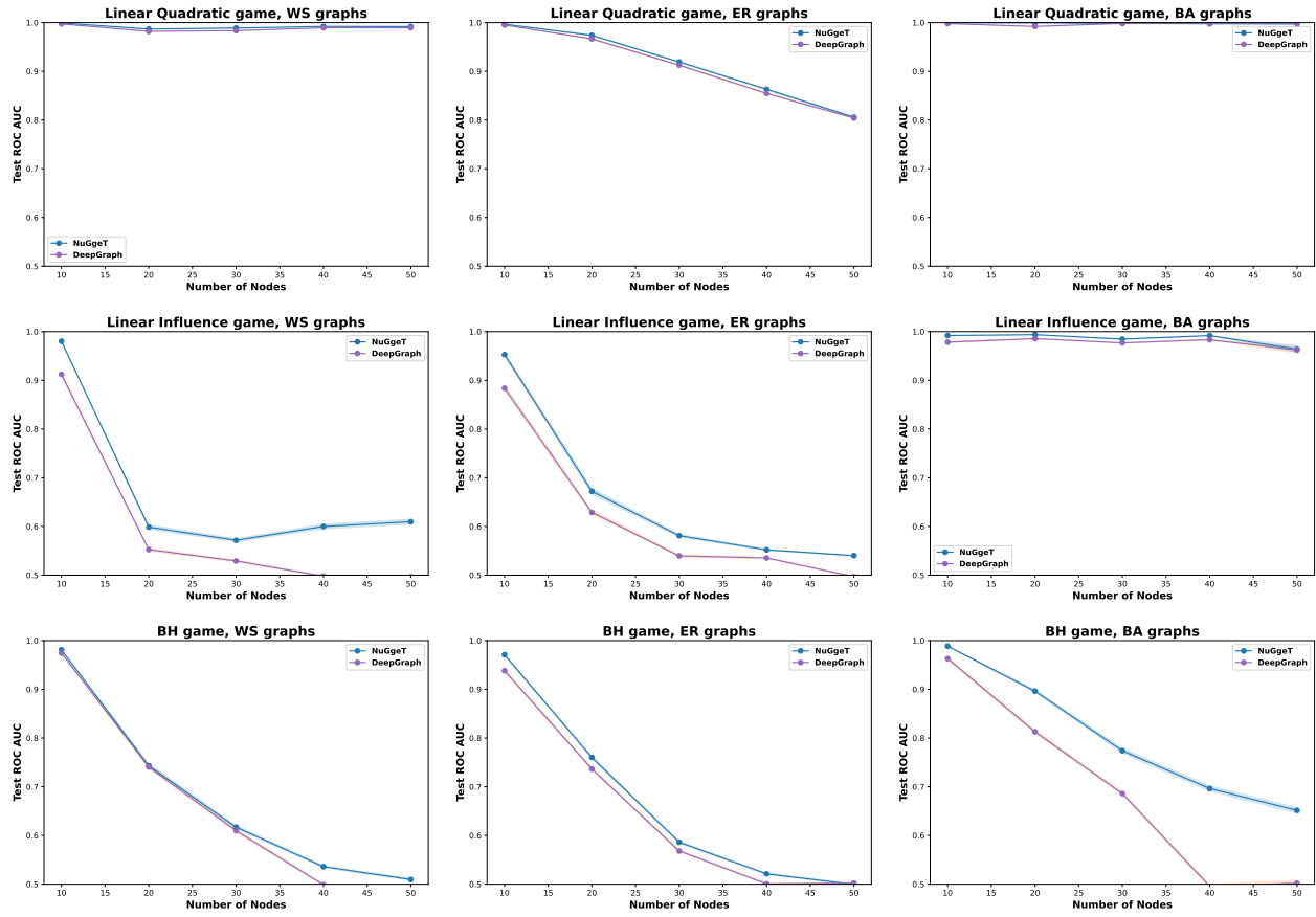
Figure 10. Results with varying number of nodes.
