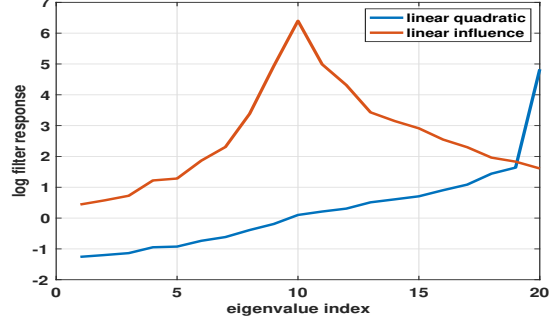
Figure 2. Interpreting actions of linear quadratic/influence games: the equilibrium actions for the two games are dominated by different sets of eigenvectors.
