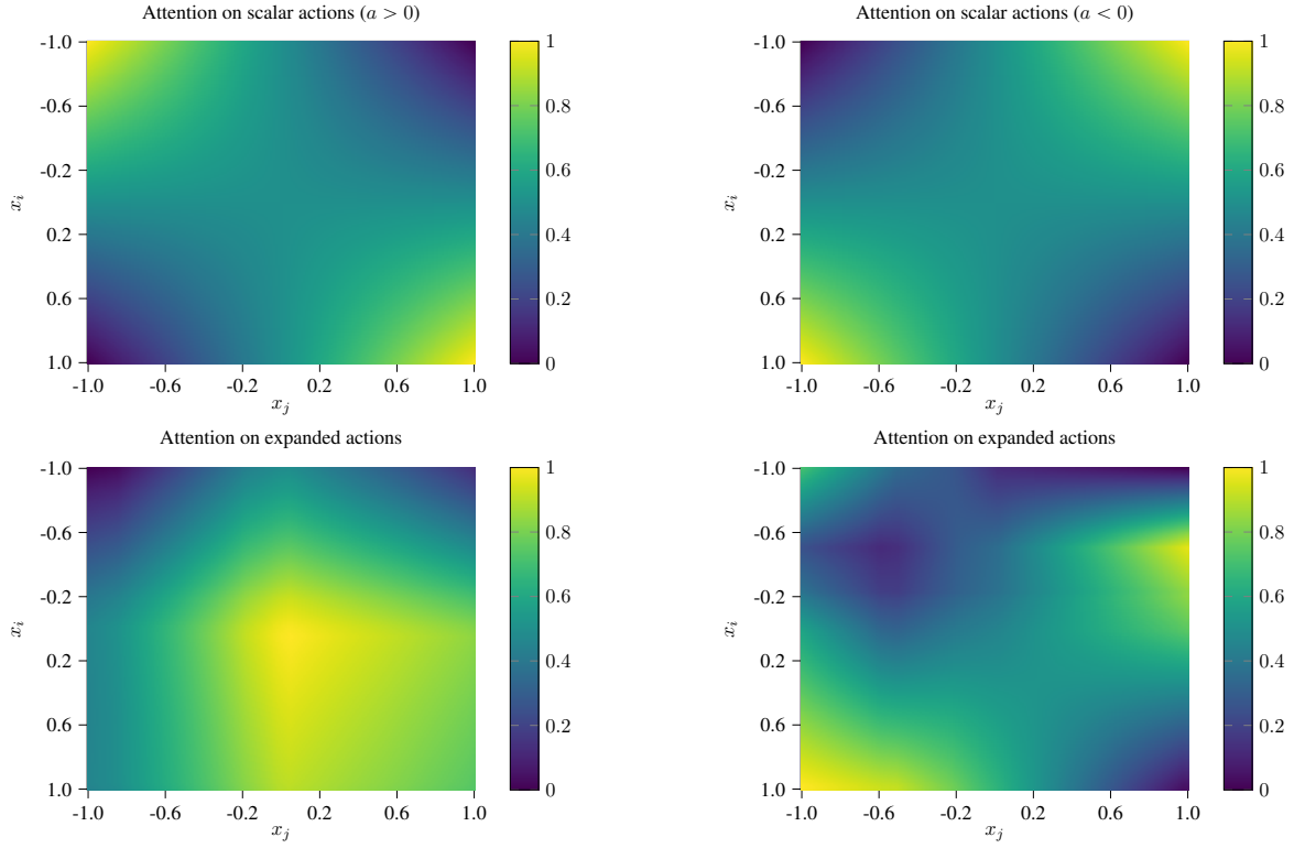
Figure 12. Top, attention values for a multiplicative attention layer directly operating on the input scalars x_i \in [-1, 1] , x_j \in [-1, 1] with positive (left) and negative (right) coefficient. Bottom, attention values for a multiplicative attention layer with random coefficients processing the expanded actions \mathbf{y}_i, \mathbf{y}_j of x_i, x_j . The result is scaled to [0, 1] for visualisation purposes.
