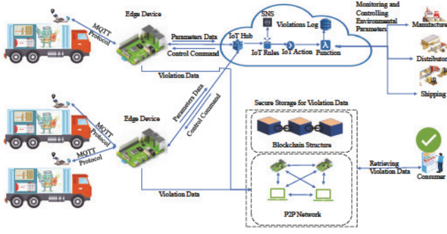
Fig. 2. Architectural Overview of Proposed PharmaChain 2.0.
