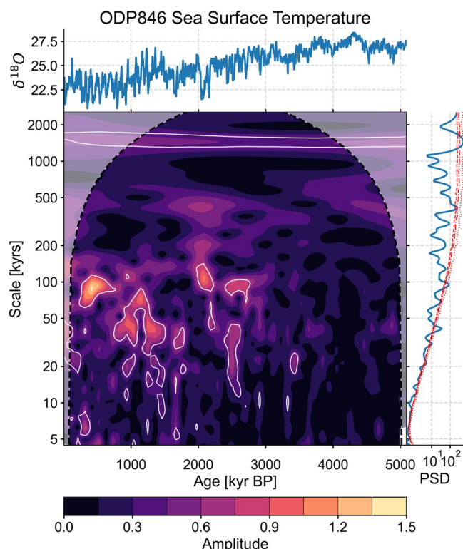
Figure 5. Summary of the spectral and wavelet analysis performed on the sea surface temperature record of Ocean Drilling Program (ODP) Site 846 (Lawrence et al., 2006). Both analyses were performed using the Weighted Wavelet Z-Transform (Foster, 1996; Kirchner & Neal, 2013) method. The record displays significant periodicities in the 40–100 kyr bands.
