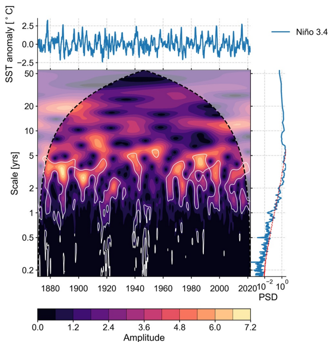
Figure 2. Summary of the spectral and wavelet analysis performed on the Niño 3.4 sea surface temperature (SST) anomalies timeseries as encoded in Pyleoclim. The series displays significant power in the 2–7 years band, consistent with the El Niño Southern Oscillation.
