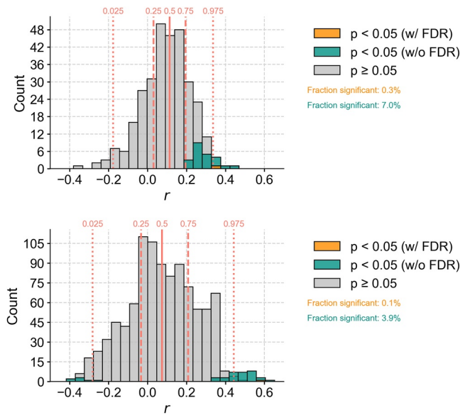
Figure 7. Ensemble correlations in Pyleoclim. Top: histogram of Pearson correlations ( r ) between the published Crystal Cave record of McCabe-Glynn et al. (2013) with the HadCRUT4 Sea surface temperature (SST) field over the North Pacific (327 grid points). Bottom: histogram of Pearson correlations ( r ) between the Crystal Cave record of McCabe-Glynn et al. (2013) with a 1000-member Bchron (Haslett & Parnell, 2008) age model ensemble with the HadCRUT4 SST at 32.5°N, 142.5°W in the Kuroshio Extension region. On both panels, “FDR” denotes the False Discovery Rate criterion of Benjamini and Hochberg (1995).
