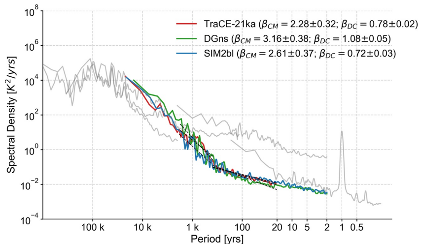
Figure 8. A spectral estimate of the global-average surface temperature variability as portrayed by transient model simulations (TraCE-21ka (Liu et al., 2009), DG ns (Meniel et al., 2011), SIM2bl (Timm & Timmermann, 2007), colors) and observational datasets (gray): HadCRUT4, The Met Office Hadley Centre gridded data set of global historical surface temperature anomalies (Morice et al., 2012); PAGES2k/LMR, the Last Millennium Reanalysis framework (Hakim et al., 2016; Tardif et al., 2019) applied to the PAGES 2k Consortium (2017); the reconstruction of global average surface temperature of Snyder (2016); ProbStack: A probabilistic Pliocene-Pleistocene stack of benthic \delta^{18}\text{O} (Ahn et al., 2017). The regional data set EPICA Dome C Ice Core 800 Kyr Deuterium Data and Temperature Estimates (Jouzel et al., 2007). \beta s denote the estimated scaling exponents over each appropriate frequency band: \beta_{\text{CM}} is the centennial-to-millennial scale exponent estimated over scales of 400–2,000 years, while \beta_{\text{DC}} is the decadal-to-centennial-scale exponent, estimated over 20–400 years.
