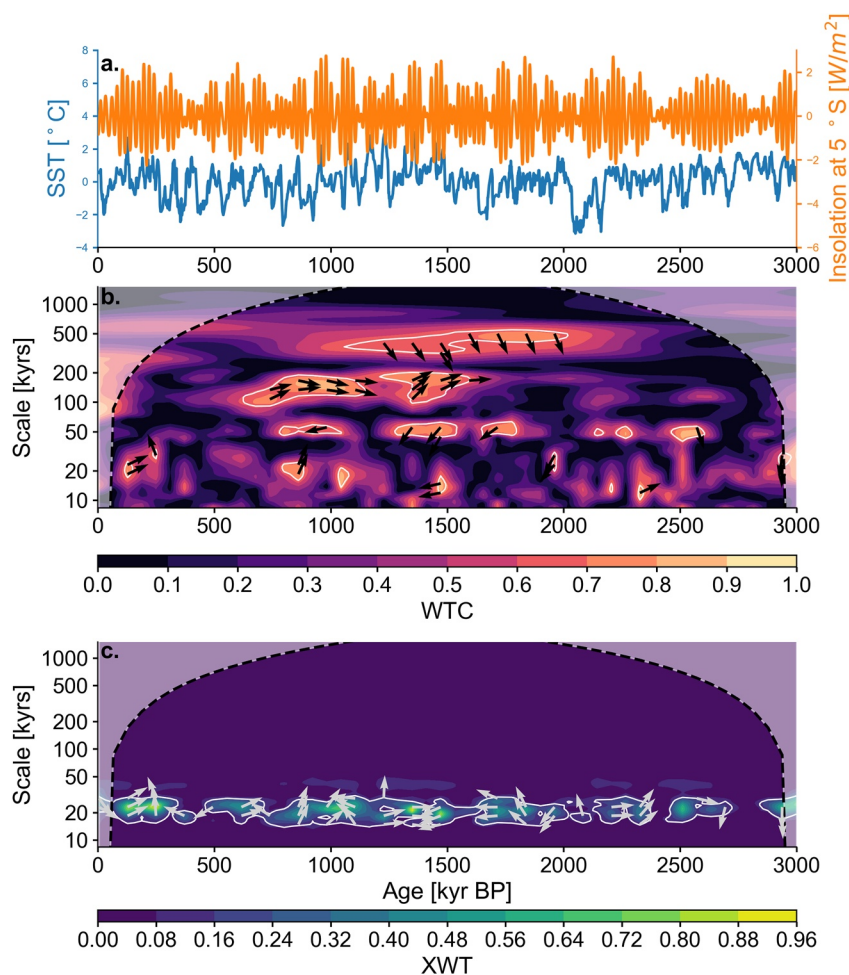
Figure 6. Coherence analysis in Pyleoclim . (a) Sea surface temperature (SST) over the past 3 million years obtained from alkenone paleothermometry at Ocean Drilling Program (ODP) Site 846 (blue) and insolation at 5°S (orange) calculated using the climlab package (Rose, 2018). (b) Wavelet transform coherence (WTC) obtained from WWZ between the two timeseries. Contours display WTC, which indicates the degree of resemblance between the signals at each time and scale. The angle of the phase arrows show the relative phasing at each time and scale (e.g., in-phase records are indicated by arrows pointing to the right, out-of-phase to the left, and in phase quadrature up and down). Phase angles are only shown for areas with significant coherence values, assessed against 1,000 random realizations of an AR(1) process. (c) Cross-wavelet transform, with contours displaying areas of high common power, and phase arrows as above. For details on the method, see Grinsted et al. (2004).
