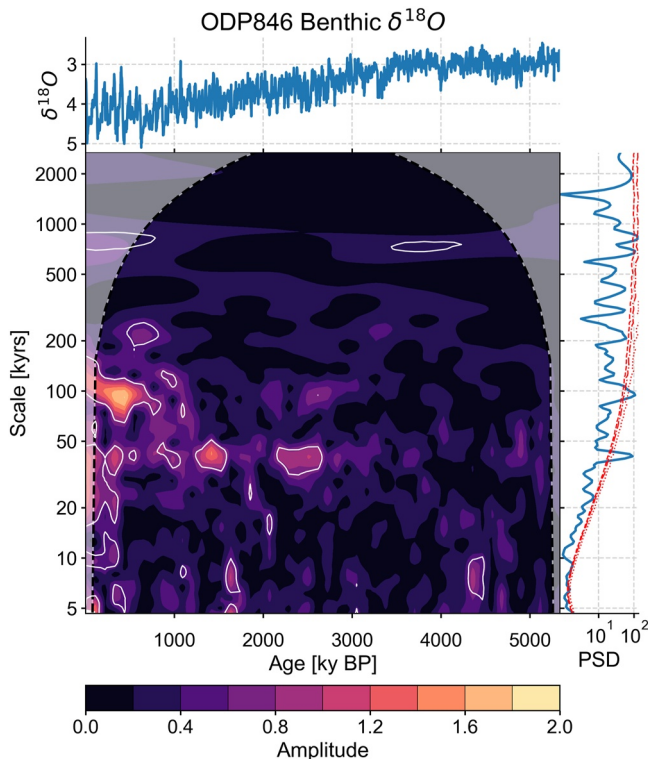
Figure 4. Summary of the spectral and wavelet analysis performed on the benthic \delta^{18}\text{O} record of Ocean Drilling Program (ODP) Site 846 (Mix et al., 1995; Shackleton et al., 1995). Both analyses were performed using the Weighted Wavelet Z-Transform (Foster, 1996; Kirchner & Neal, 2013) method. The record displays significant periodicities in the 40 and 100 kyr bands with a drop in power in the 100 kyr band at the mid-Pleistocene transition.
