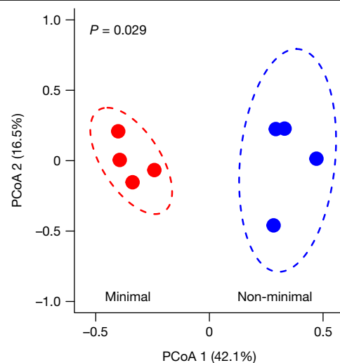
Fig. 3 | The non-minimal cell and minimal cell populations acquired adaptive mutations in different sets of shared genes. Ordination from a principal coordinates analysis (PCoA) created by a gene-by-population matrix using the Bray–Curtis distance metric after 2,000 generations of evolution (Extended Data Tables 2–4). The dashed lines represent 95% confidence ellipses around replicate populations ( n = 4 for each cell type) represented by dark coloured symbols.
