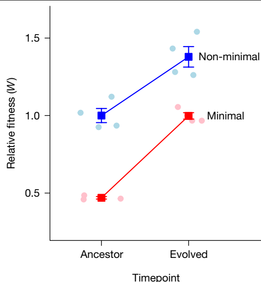
Fig. 2 | The effect of genome minimization on fitness and adaptation.
