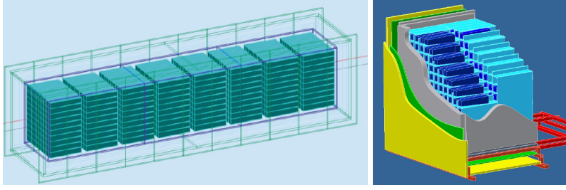
Figure 1: Left: schematic of the BDX experimental setup (see text). Right: sketch of the BDX detector, showing the full reference design composed of 8 modules of 10 \times 10 CsI(Tl) crystals.
