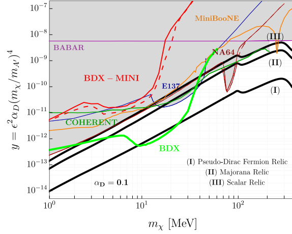
Figure 4: BDX-MINI exclusion limits assuming \alpha_D = 0.1 and m_{A'} = 3m_\chi for scalar LDM (continuous red line) and fermionic LDM (dashed red line), compared with the full BDX experiment sensitivity (green line). The thick black lines represent the relic target. The other colored lines show the current most stringent exclusion limits from other experiments (see e.g. [3] for further details)
