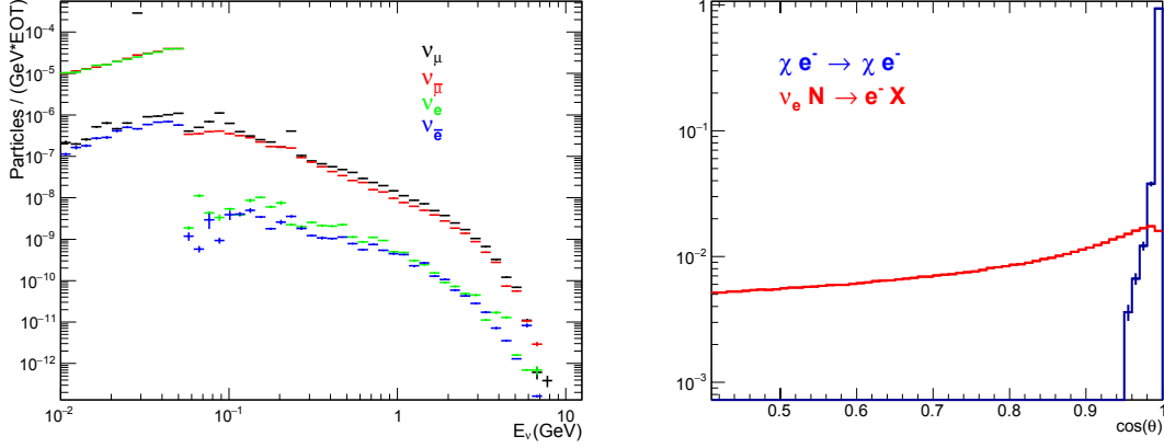
Figure 2: Left: differential energy spectrum of neutrinos impinging on the BDX detector. Right: scattered electron angle distribution for the signal ( e^- \chi \rightarrow e^- \chi ) and \nu_e CC background ( \nu_e N \rightarrow e^- X ) reactions. The two histograms have been normalized to the same area.
