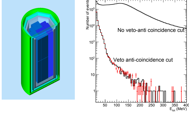
Figure 3: Left: GEANT4 rendering of the BDX-MINI detector, showing the \text{PbWO}_4 crystals (blue), the tungsten shielding (gray), the IV (cyan) and the OV (green). Right: in black, the calorimeter energy distribution for the beam-on data sample with and without the veto anti-coincidence cut. In red, the beam-off anti-coincidence data sample, properly normalized in time.
