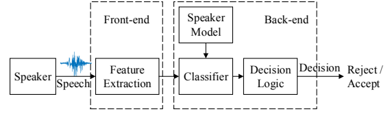
Fig. 2: Automatic speaker verification (ASV) system
