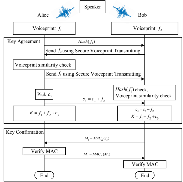
Fig. 4: Voiceprint-based key agreement
