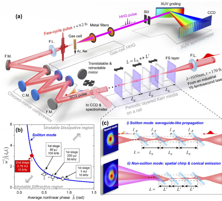
Fig. 1. (a) Schematic of the experimental setup. The long femtosecond pulse is focused into PLKM for SCG. A translatable and retractable mirror is used to deflect the beam for monitoring the spectra and beam profiles in the far field, from which the appropriate condition L = L_R can be determined. The HHG is generated by focusing the compressed pulses into a gas cell. F.L.: focusing lens; F.M.: folding mirror; C.M.: chirped mirror. (b) The universal relationship between the normalized beam radius squared, i.e., \bar{w}^2/(\lambda_0 L) , and the average nonlinear phase \bar{b} for the soliton modes predicted by the FKD-FLI model [46]. The symbols are the experimental results under different conditions. (c) The illustrations of the beam propagation under i) the soliton mode and ii) the non-soliton mode under different L . When L is short, conical emission and spatial chirp can be clearly observed.
