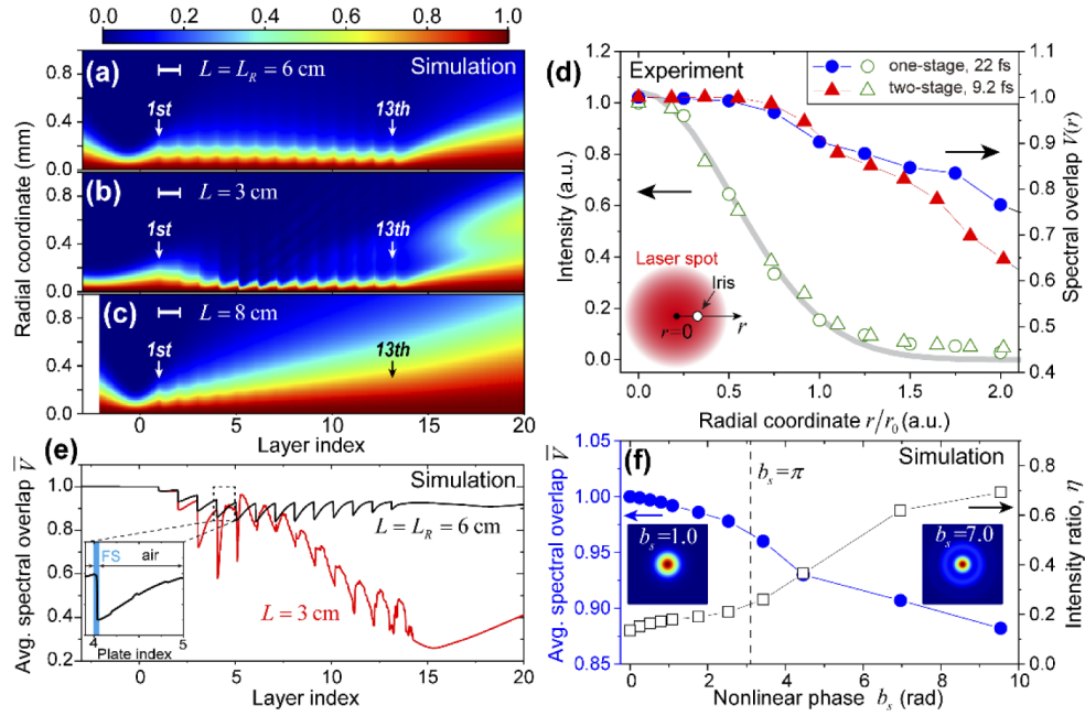
Fig. 3. (a)-(c) The variation of the beam radial intensity as the beam propagates through the PLKM with L = 6 cm ( L_R ), 3 cm and 8 cm, respectively, obtained from the NLSE simulations. (d) The beam intensity and spectral overlap V(r) along the radial coordinate r for the compressed pulses under the optimum conditions of the one-stage ( \sim 22 fs) and two-stage ( \sim 9.2 fs) compressors. The grey solid line represents the Gaussian fitting to the intensity profile. Inset: illustration of the spatial-filtering experimental setup. (e) The evolution of the average (avg.) spectral overlap integral, \bar{V} , obtained from the NLSE simulations. The simulation conditions are the same as (a) for L = 6 cm and (b) for L = 3 cm. Inset: the zoom-in view of the \bar{V} variation within and after a single FS plate. (f) The NLSE simulations of \bar{V} and the intensity ratio \eta after the laser beam passes through a single FS plate with l = 800 \mu\text{m} . Inset: the spatial modes of the output beam with b_s = 1.0 and 7.0 rad.
