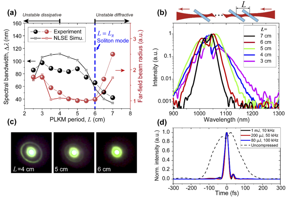
Fig. 2. (a) The spectral bandwidth and the normalized far-field beam radius as a function of the PLKM period L obtained from our experiments and NLSE simulations (simu.). The PLKM is composed of 13 FS layers with l = 800 \mu\text{m} . The input pulse energy is 200 \mu\text{J} at 50 kHz. The soliton mode can be identified and labelled by the blue dashed line. (b) The experimentally measured on-axial spectra of the output beam under different L corresponding to (a). (c) The far-field spatial mode of the output beam measured by a laser viewing card (Thorlabs, VRC4) and the images are taken by a commercial camera. (d) The temporal intensity profiles of the compressed pulses under different laser conditions (1 mJ, 10 kHz; 200 \mu\text{J} , 50 kHz; 80 \mu\text{J} , 100 kHz). The dashed line represents the uncompressed pulse from the laser.
