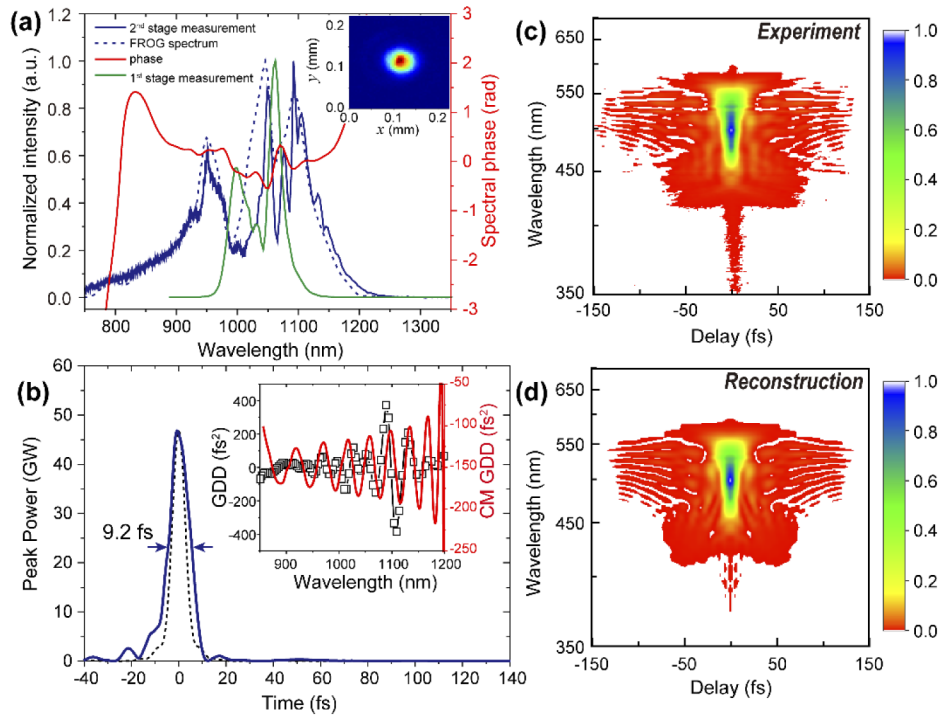
Fig. 4. (a) The measured spectrum, the FROG-retrieved spectrum and the retrieved phase of the few-cycle pulses from the two-stage compressor. The spectrum from the first-stage compressor is also shown as the green line for comparison. Inset: the beam profile of the few-cycle pulses after the focus. (b) The reconstructed intensity profile of the few-cycle pulses after the two-stage compressor with L = 9.5 cm. The TL pulse profile is plotted as the dashed line. Inset: The comparison of the GDD oscillations of the FROG-retrieved spectral phase and of the chirped mirrors (CM). (c) and (d) The measured and reconstructed FROG traces for the few-cycle pulses.
